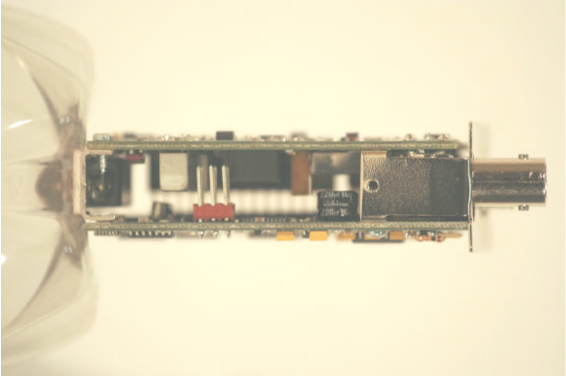
Combined RF Board and Modem Board
