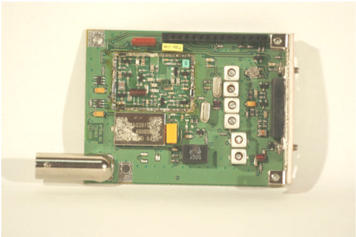
RF Board-Top View
