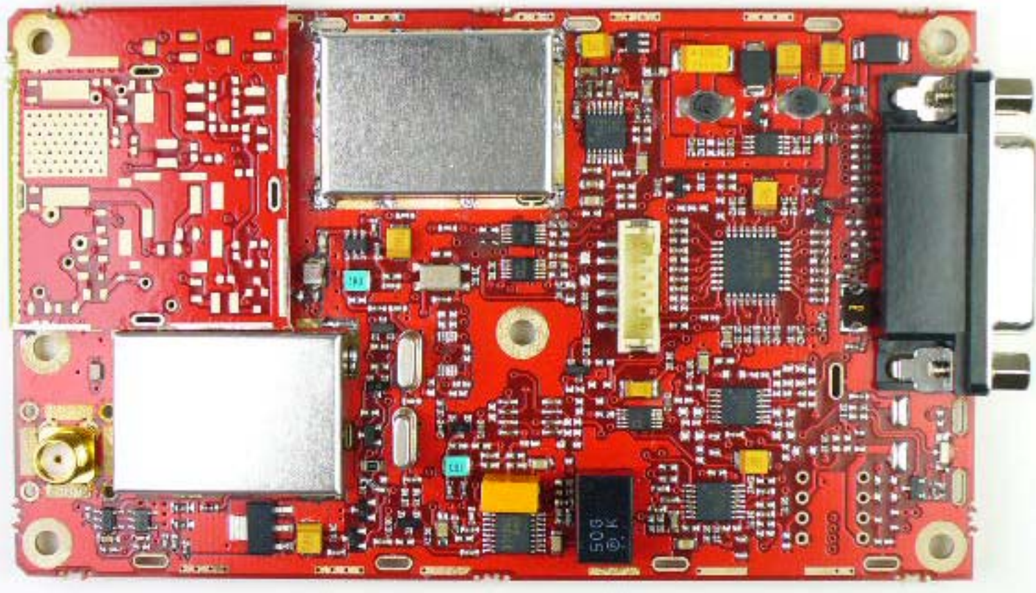
DR-445 top side with shields
