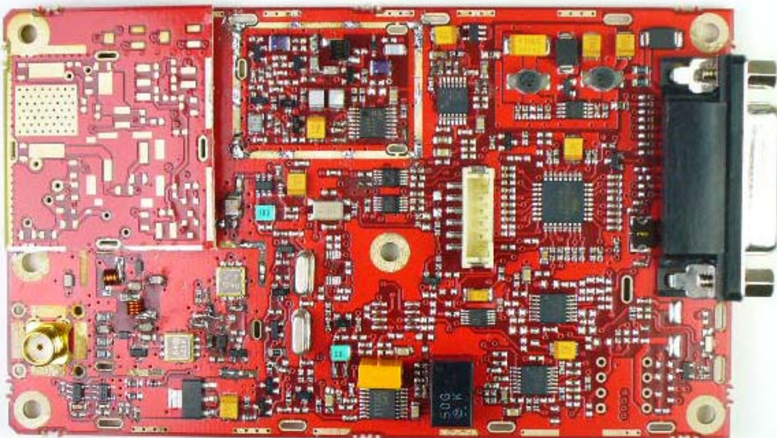
DR-445 top side with no shields
