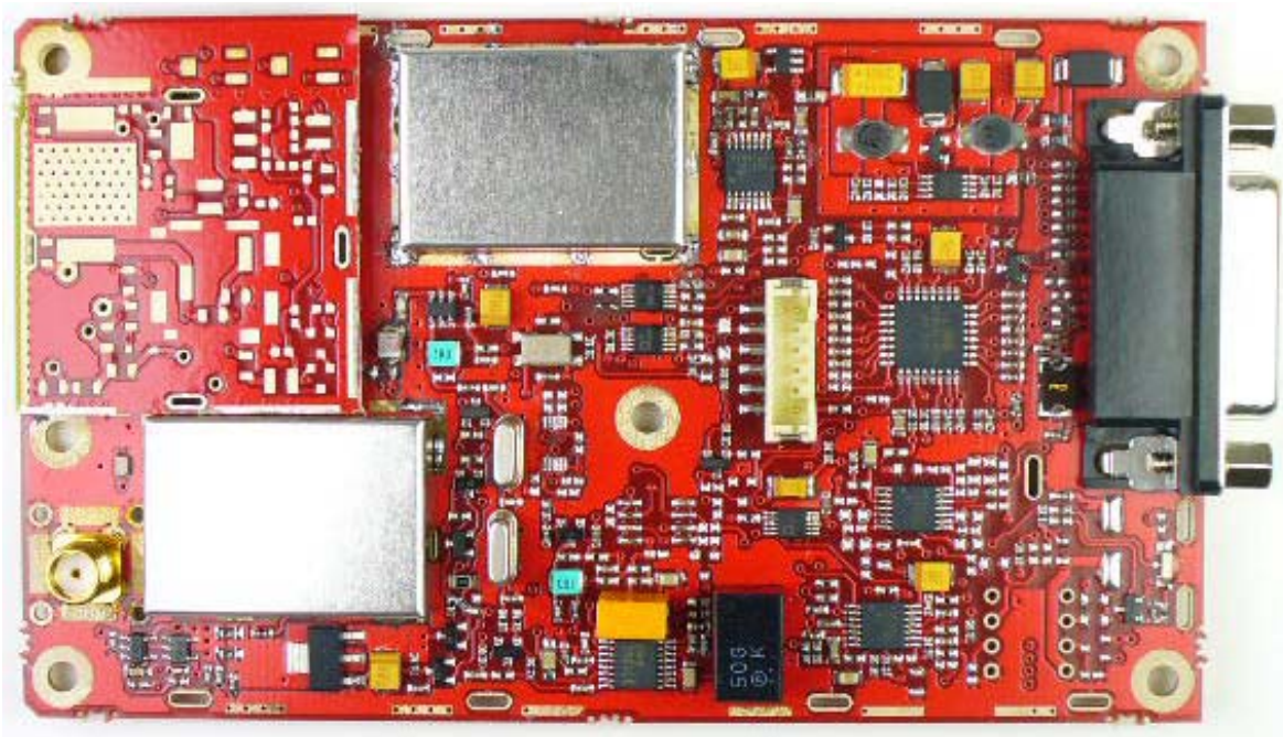
DR-445 top side with shields
