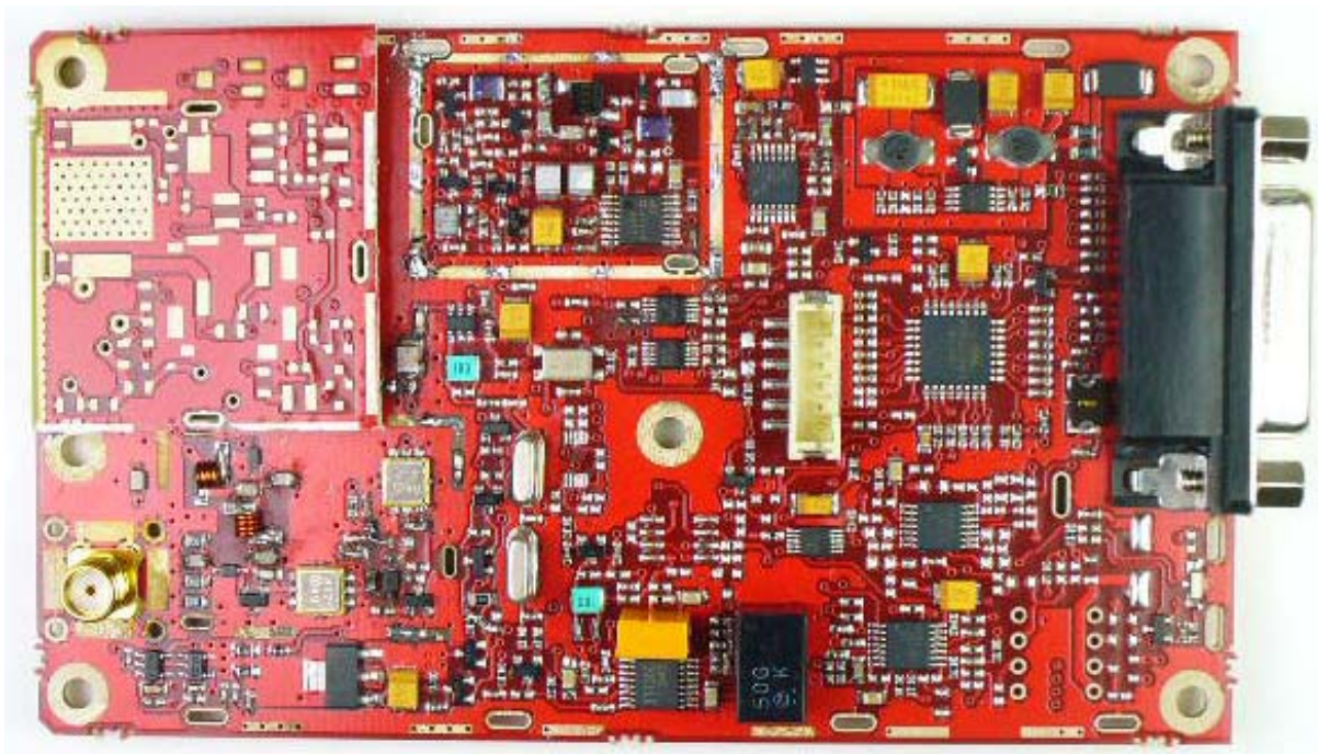
DR-445 top side with no shields
