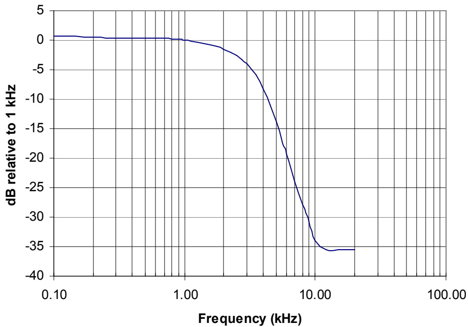
TX LPF Respns (dB)
