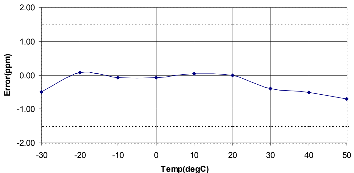
Error vs Temperature
