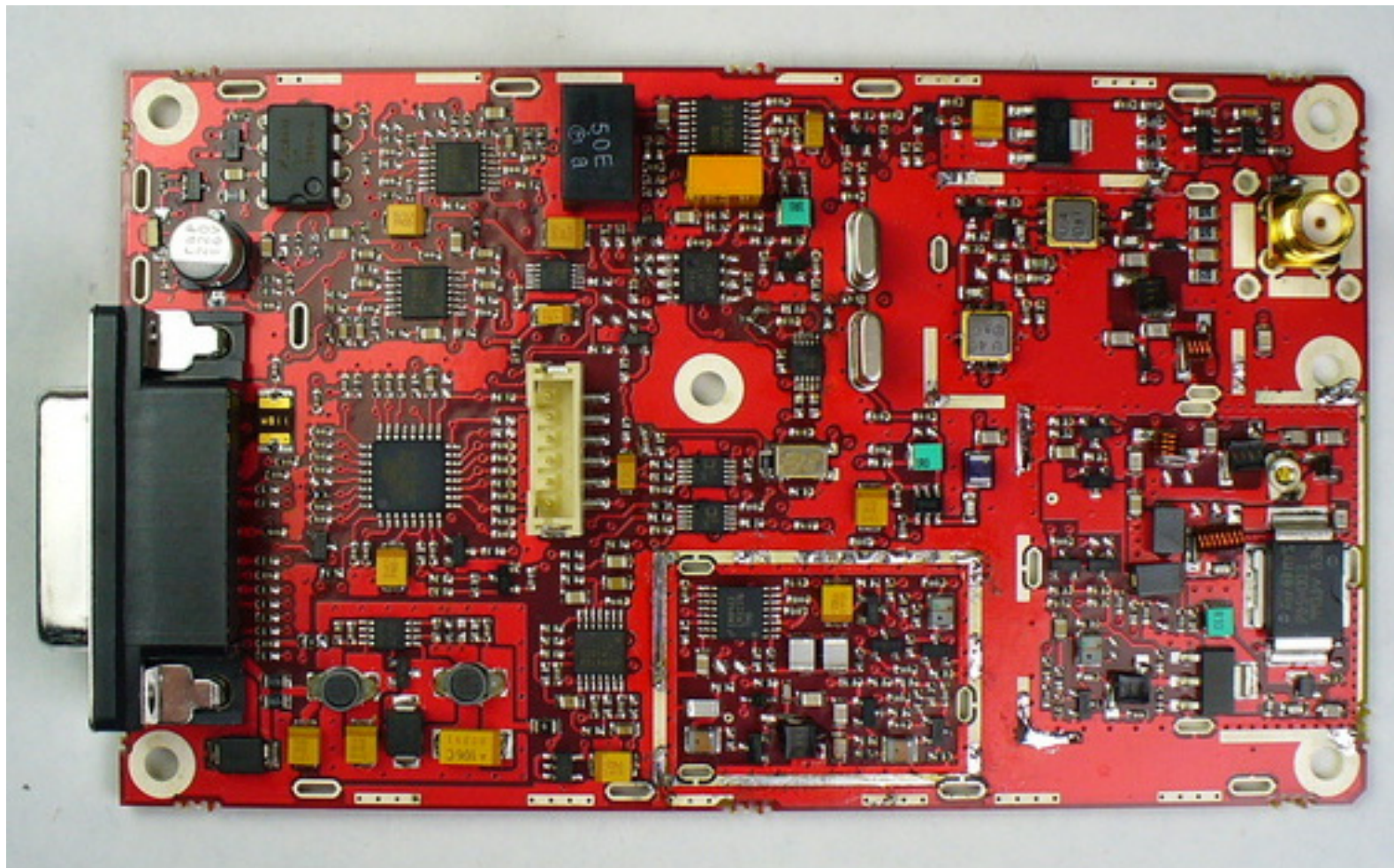
DTX-445 top side with no shields
