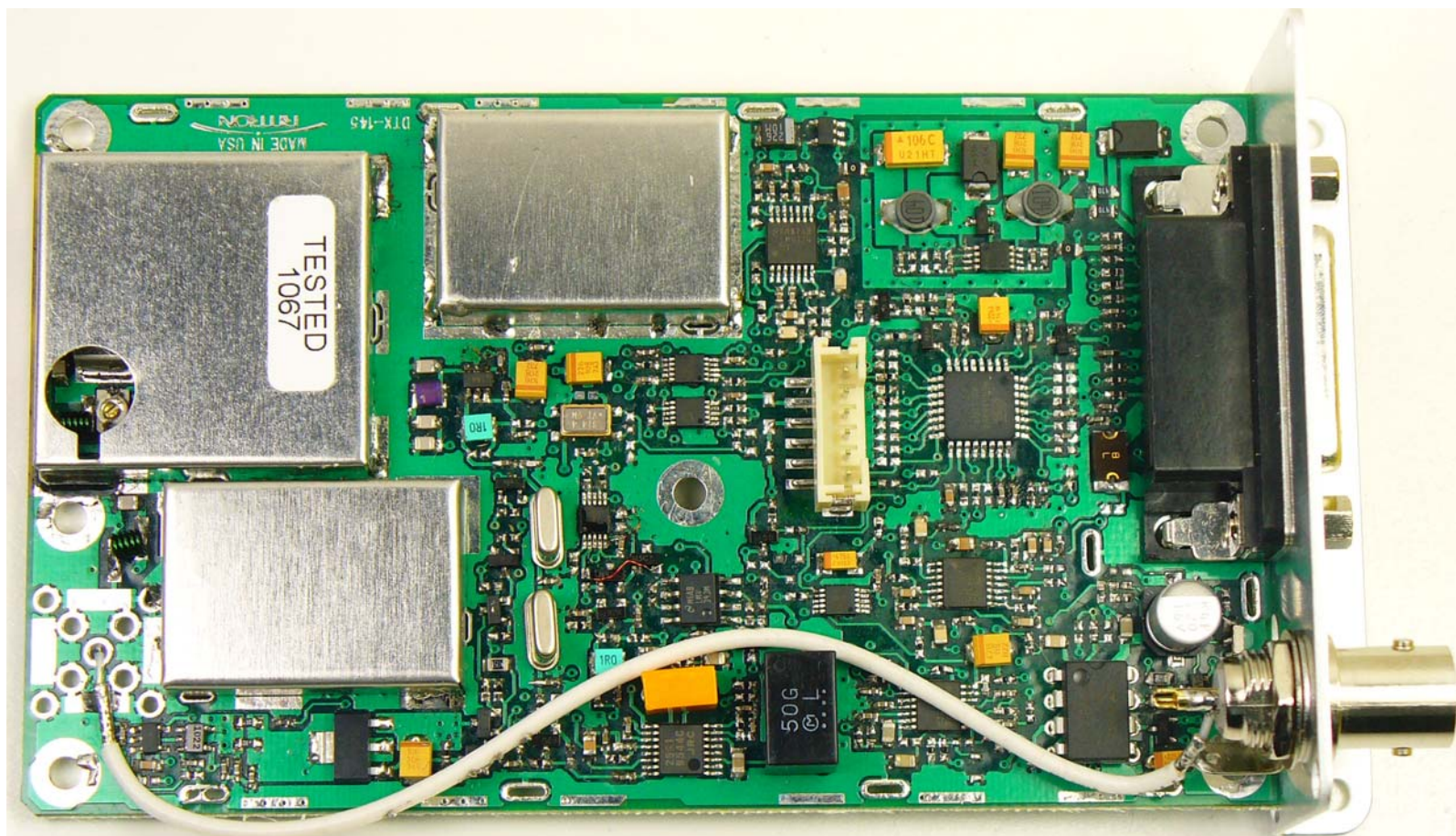
DTX-145 top side with shields
