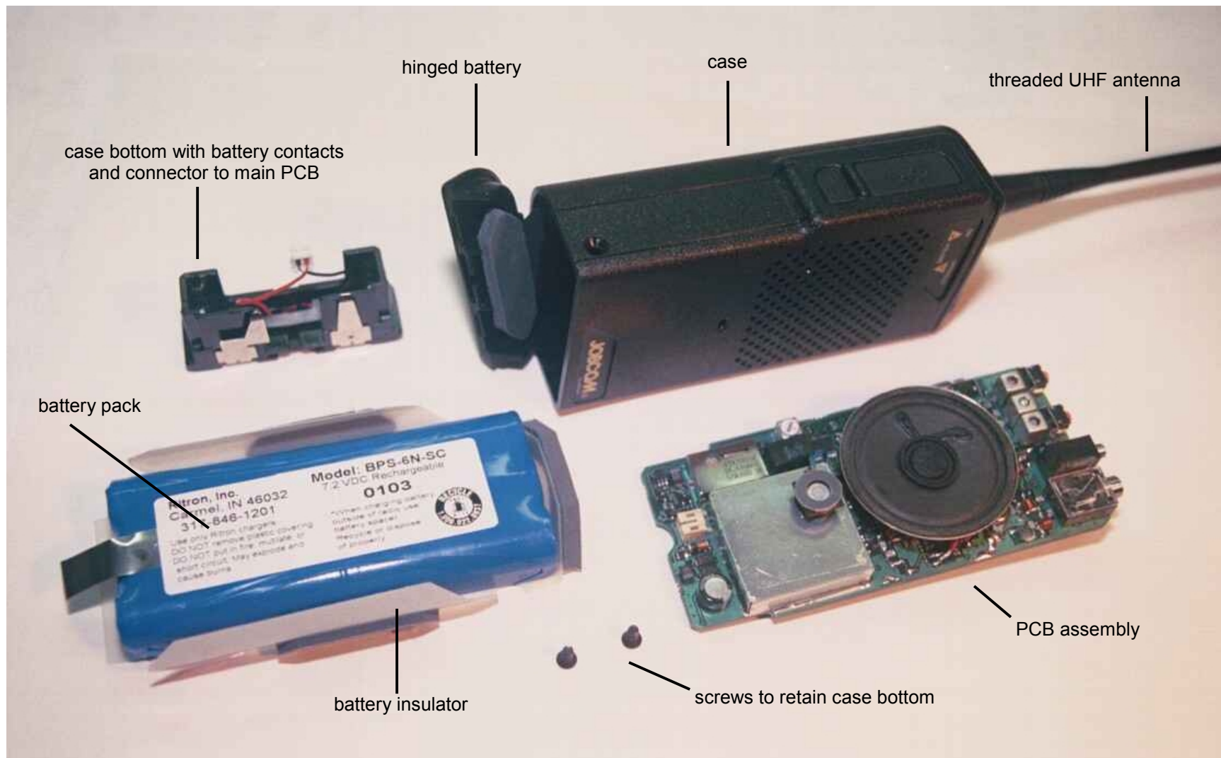
AIERIT13-442 SST-442 case assembly components
