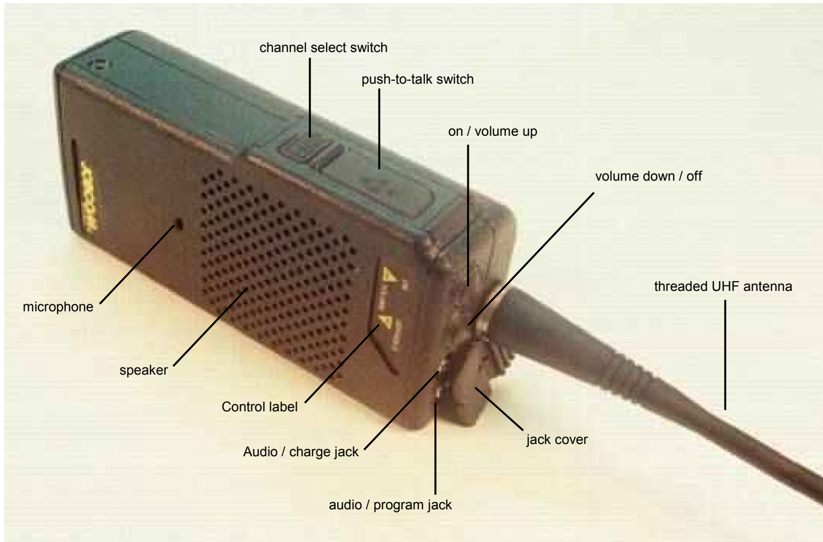
AIERIT13-442 SST-442 controls, jacks, and control label
