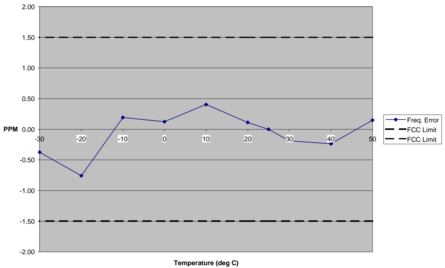
Frequency Error vs Temperature
