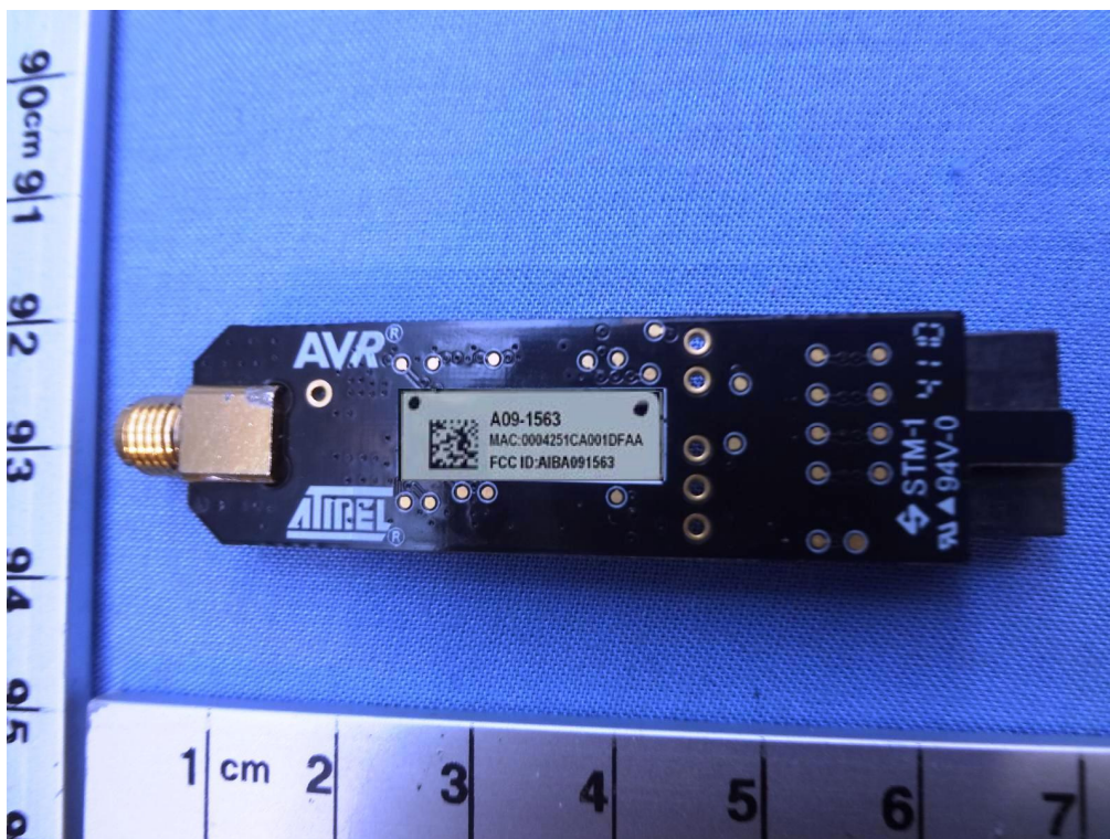
Internal of PCB Back View
