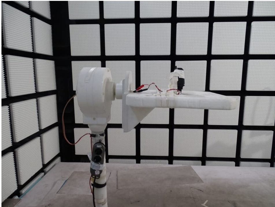
Photo 1: RSE setup 9 kHz to 30 MHz and > 1 GHz
