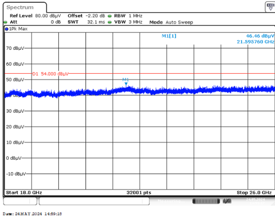
Plot 7: 18 GHz to 26 GHz, TX mode, valid for all channels and modulations
