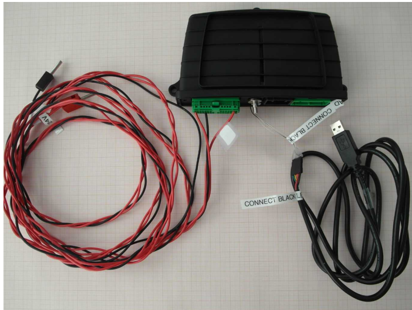
Photo 7 DUT assembly
