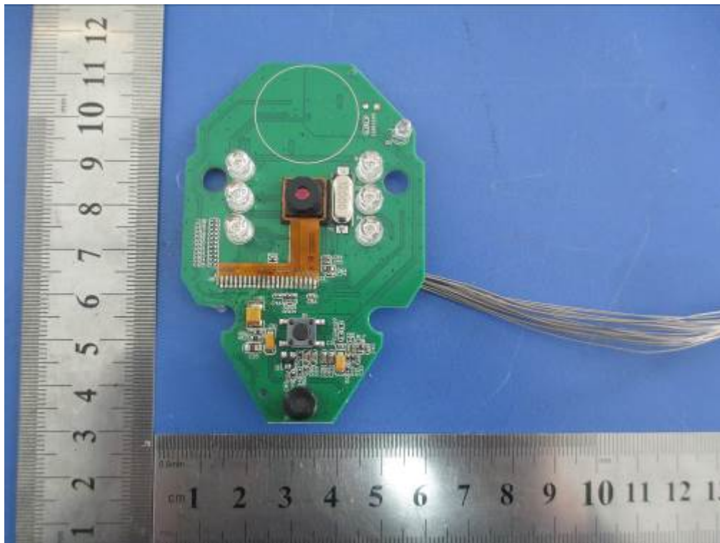
Pedestel PCB - Front View
