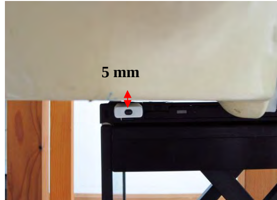
Fig.4 EUT Horizontal down mode to flat phantom
