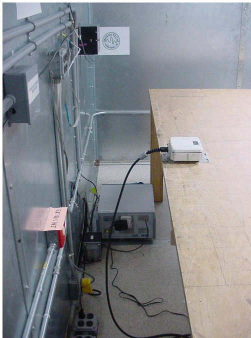
PHOTOGRAPH 4: CONDUCTED TEST CONFIGURATION (REAR VIEW)
