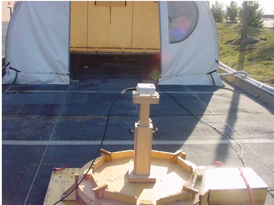
PHOTOGRAPH 1: RADIATED TEST CONFIGURATION (FRONT VIEW)
