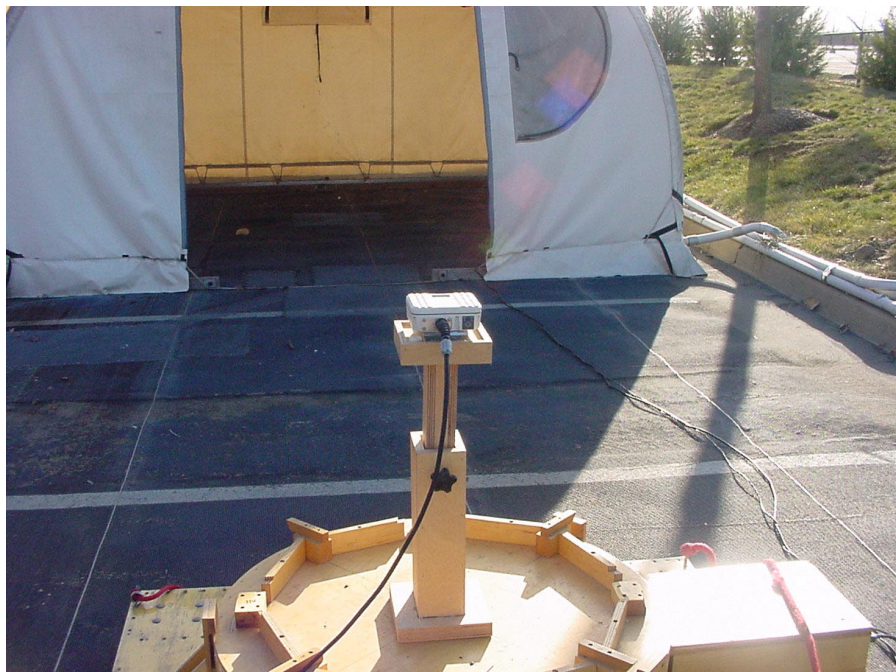
PHOTOGRAPH 2: RADIATED TEST CONFIGURATION (REAR VIEW)
