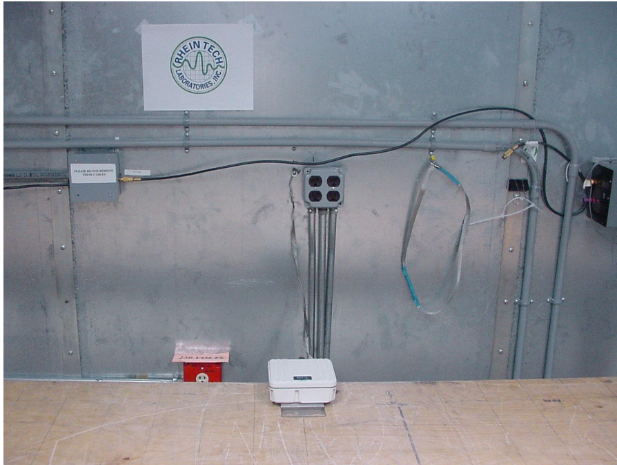
PHOTOGRAPH 3: CONDUCTED TEST CONFIGURATION (FRONT VIEW)
