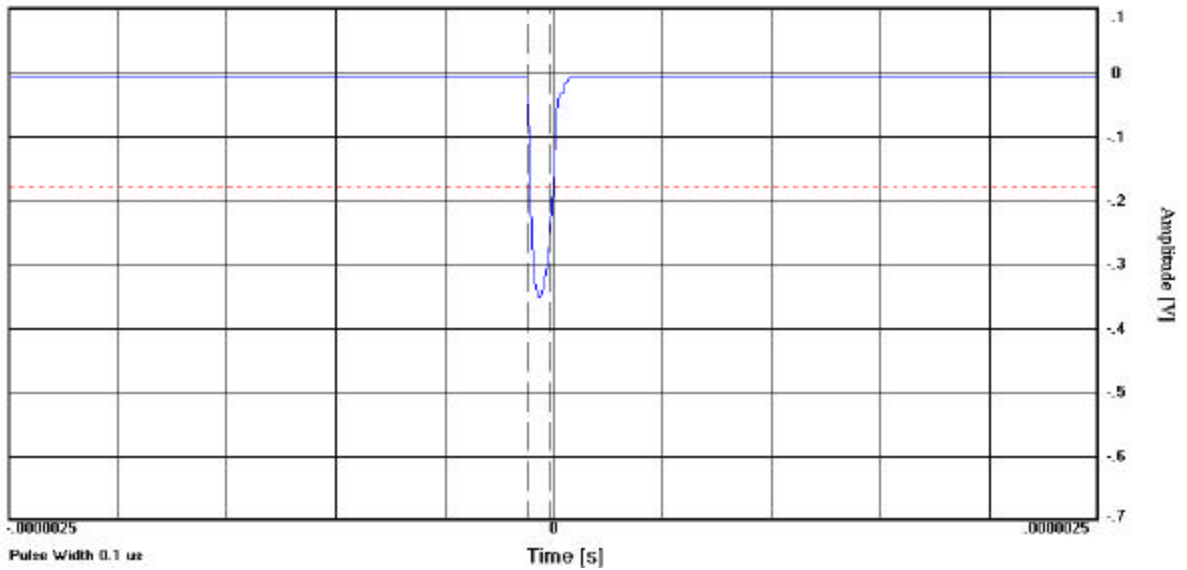
PLOT 9: MAGNETRON CONTROL PULSE 0.1µS
