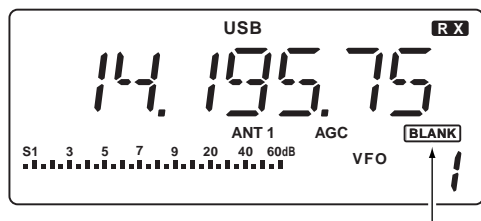
"BLANK" appears above the memory channel readout until [MW] is pushed for 2 sec.
