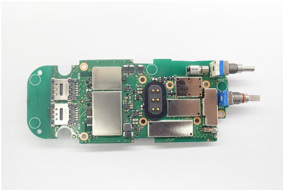
MAIN Board side-B view
