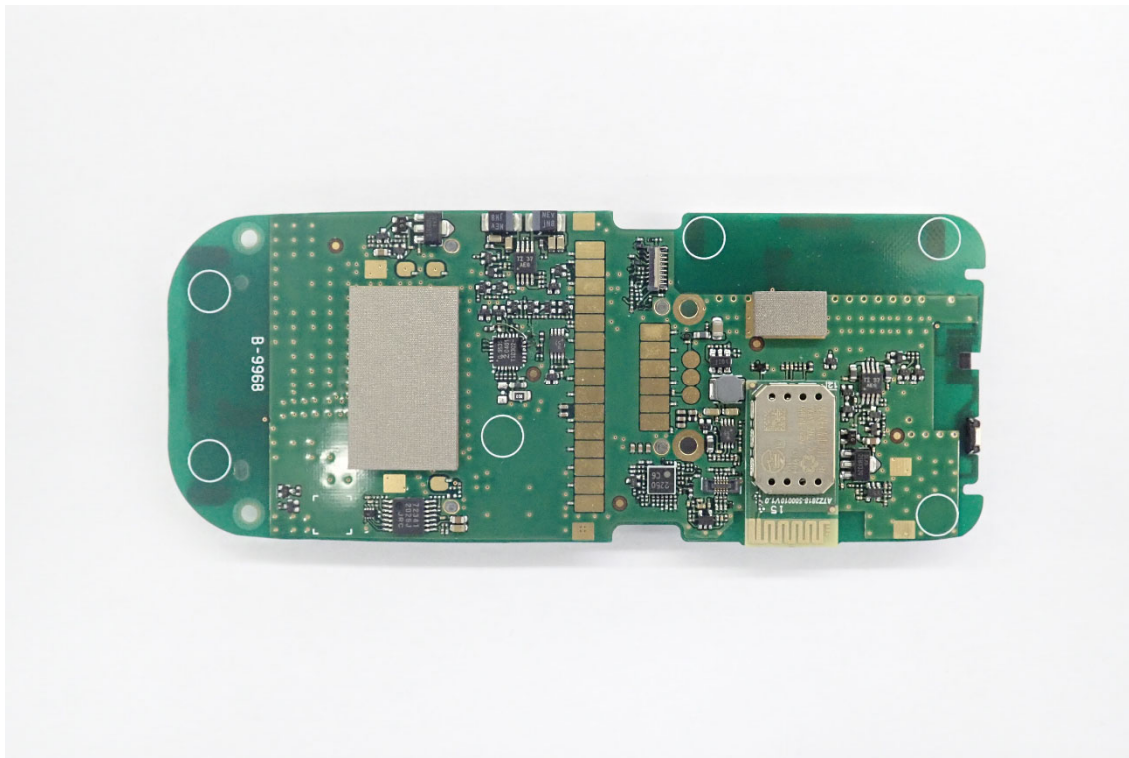
FRONT Board side-B view
