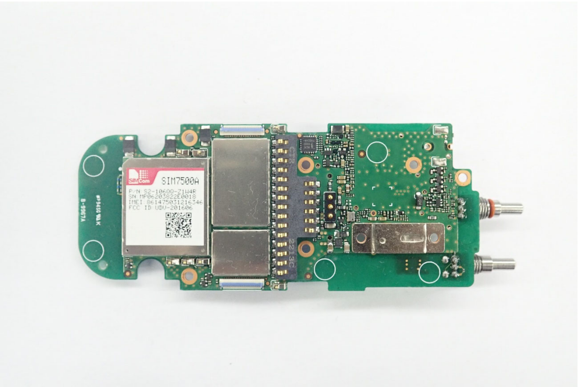
MAIN Board side-A view
