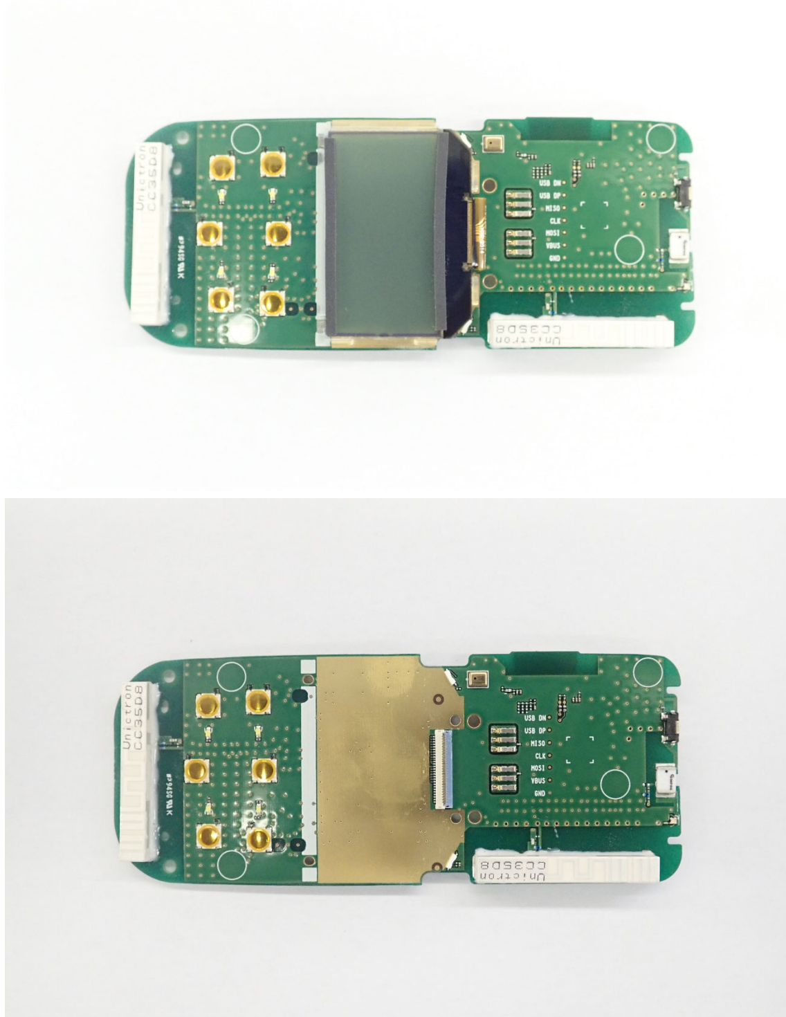
FRONT Board side-A view
