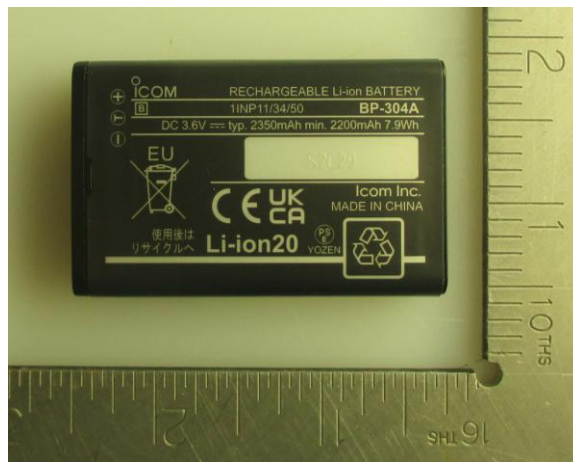
< BP-304A Battery >
