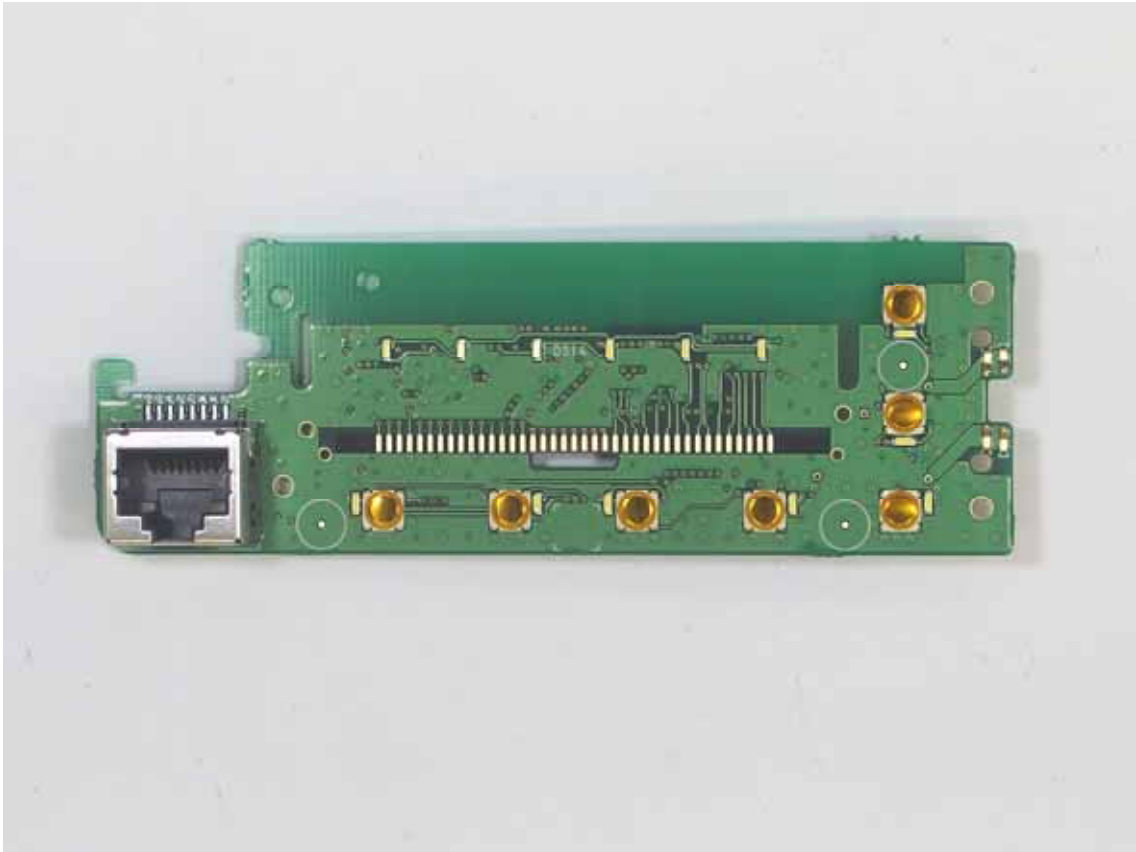
IC-F5130D Front board side-A
