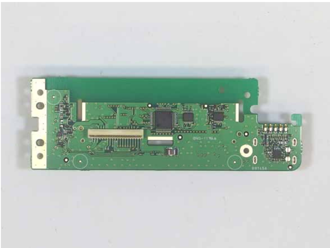
IC-F5130D Front board side-B
