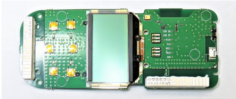
Front Board side-A view
