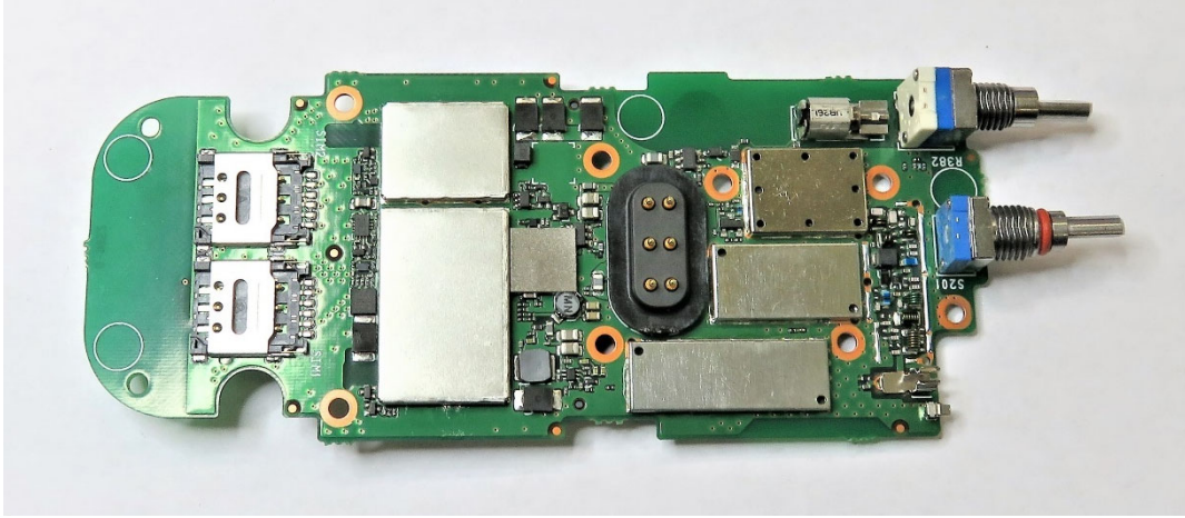
MAIN Board side-B view
