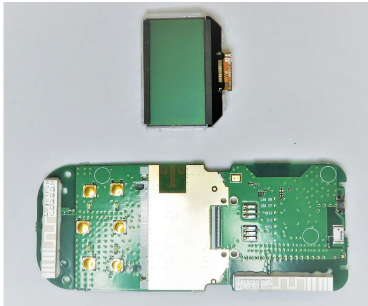
Front Board side-B view
