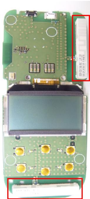
Front Board side-A view
