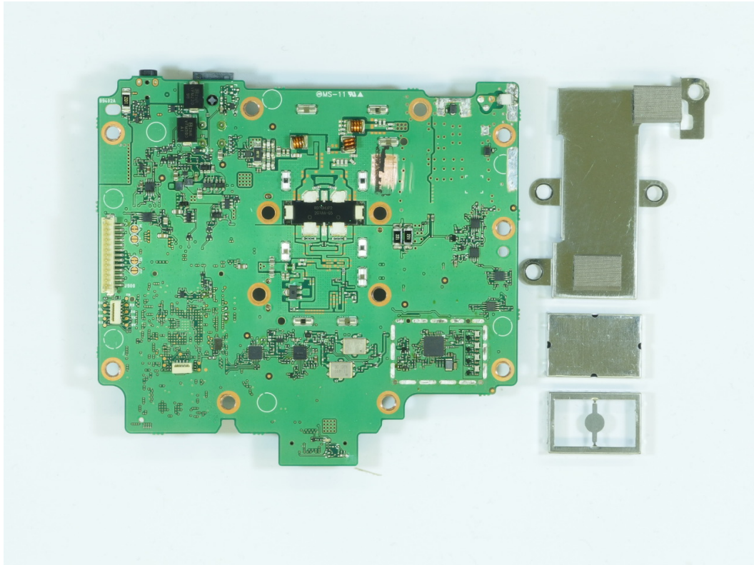
IC-F5330D MAIN unit Main board side-A
