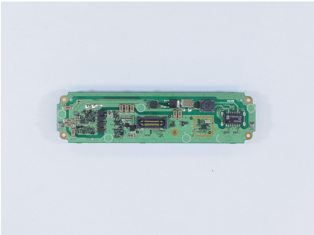
IC-F5330D MAIN unit Front board side-B
