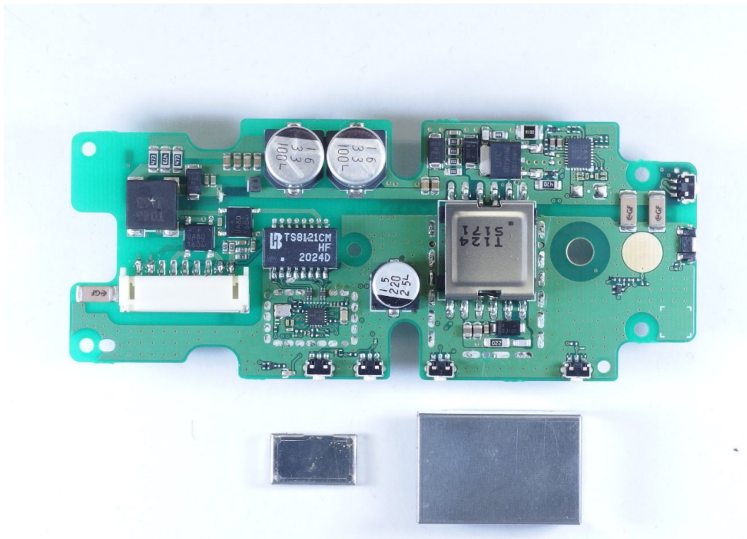
IC-F5330D MIC unit PD board side-B
