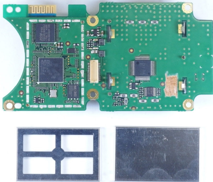
IC-F5330D MIC unit Logic board side-B
