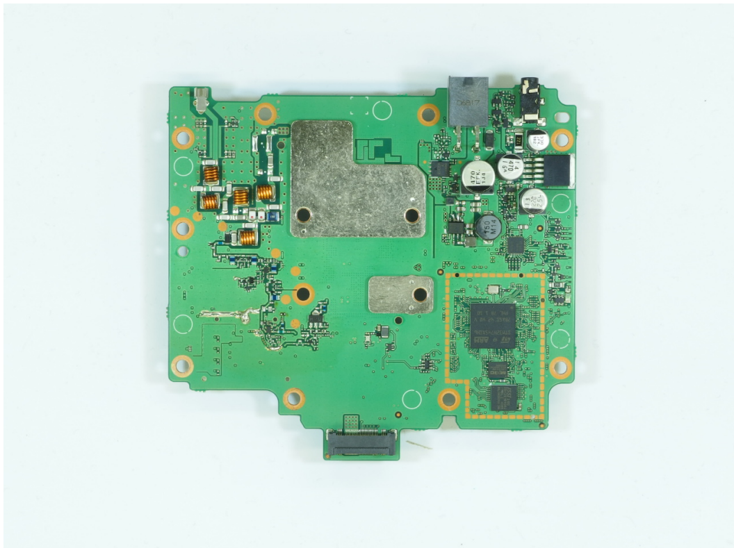
IC-F5330D MAIN unit Main board side-B
