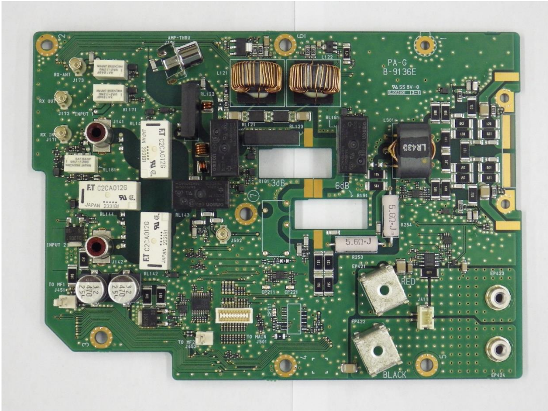
PA-G_sideA
