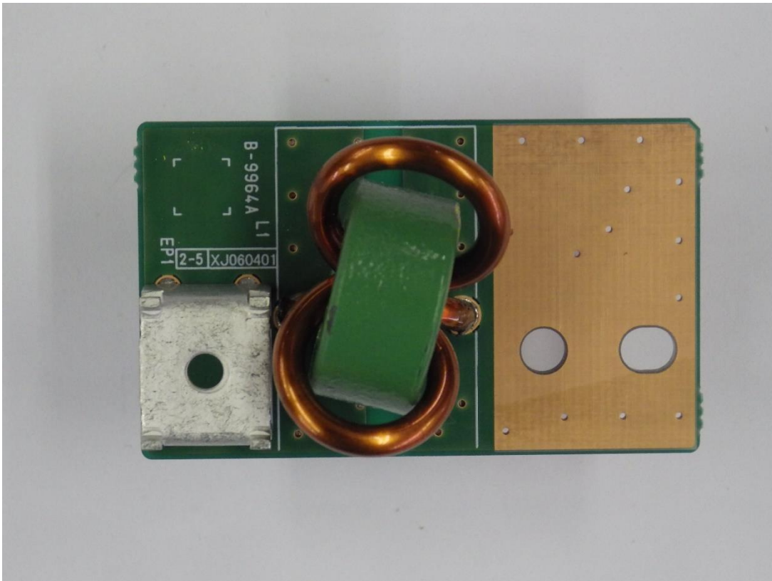
LINE-FILTER_sideA
