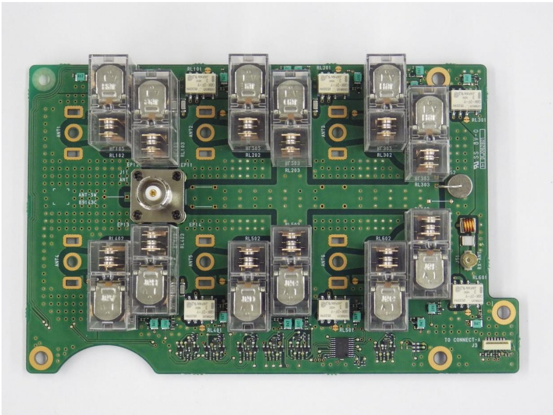
ANT-SW_sideA
