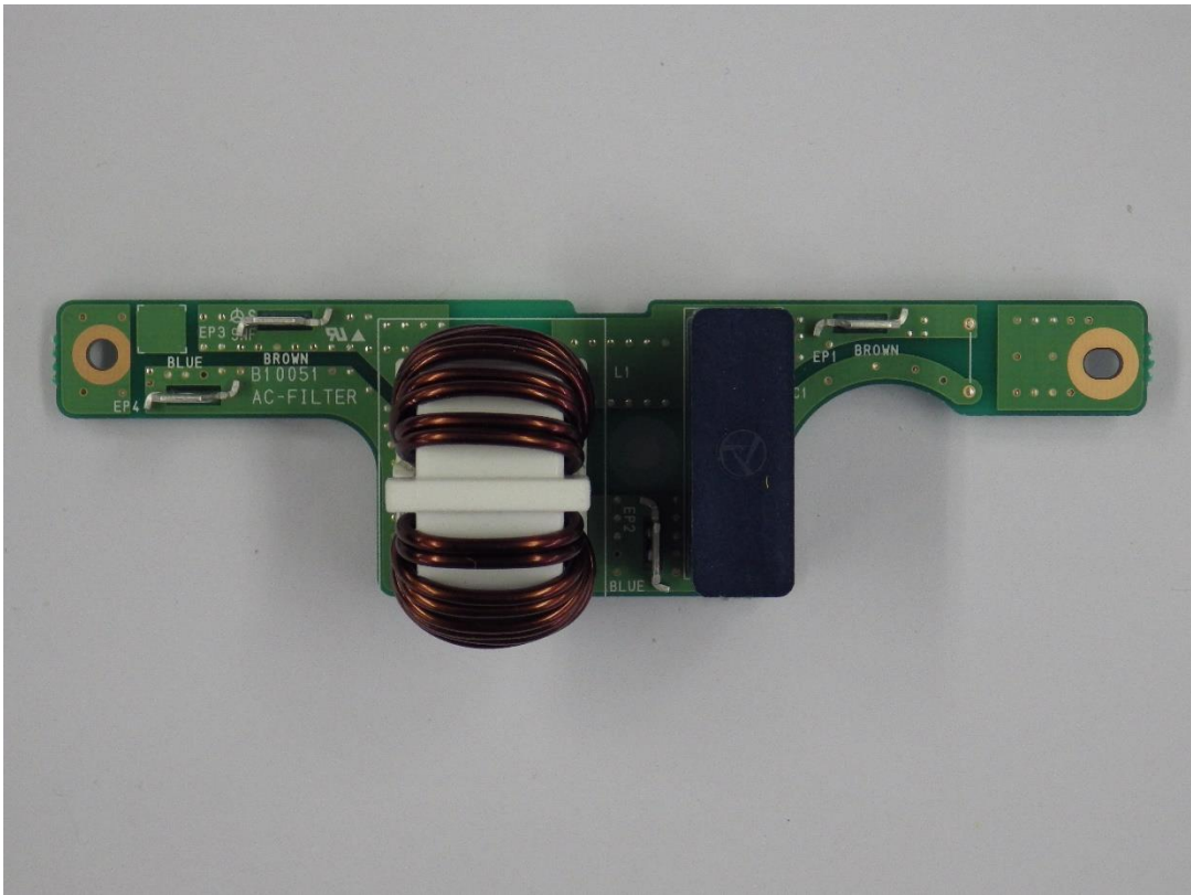
AC-FILTER_sideA
