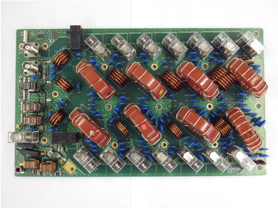
FILTER_sideA
