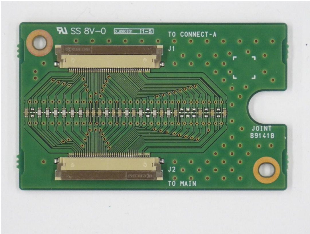
JOINT_sideA
