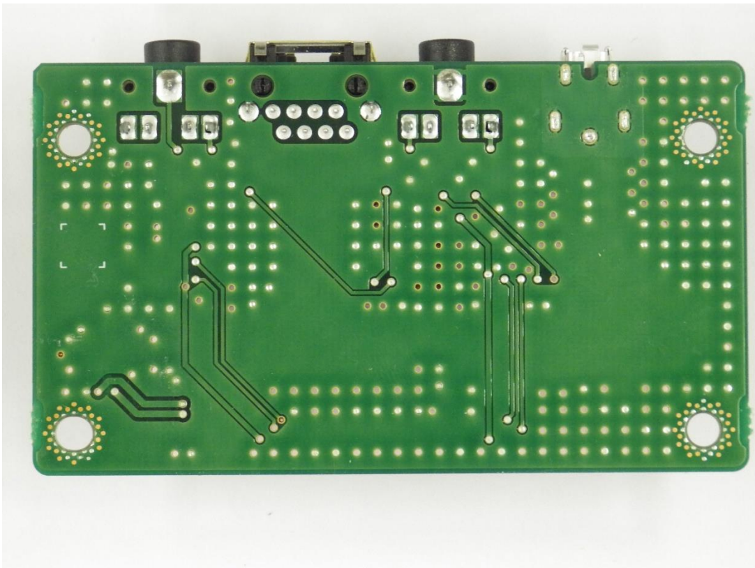
CONNECT-B_sideB
