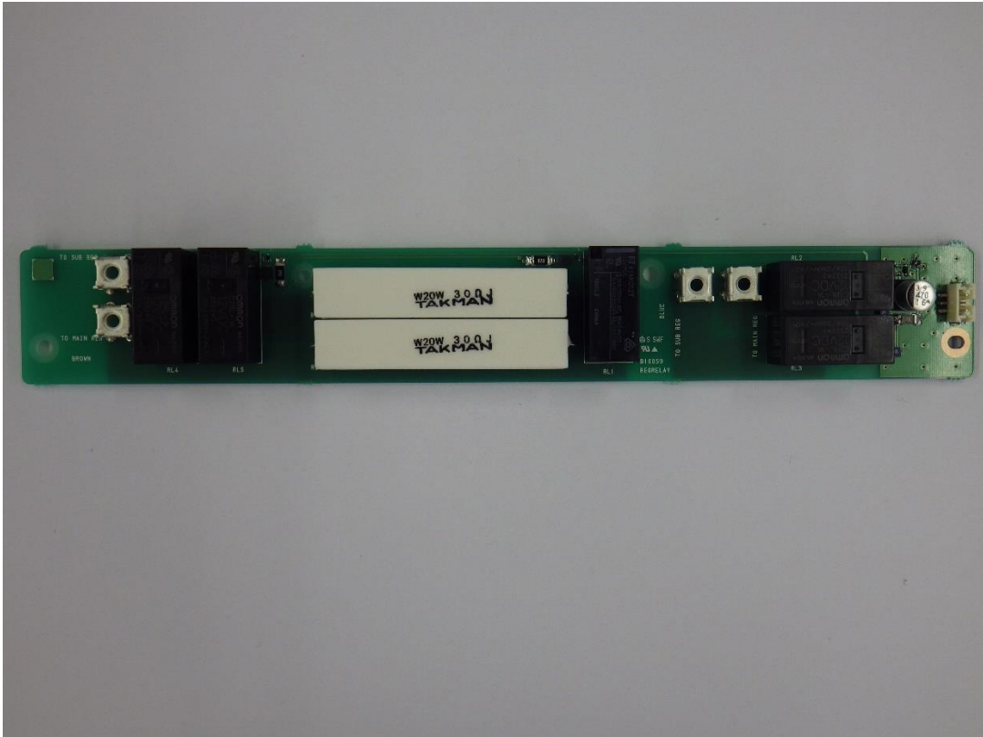
REGRELAY_sideA
