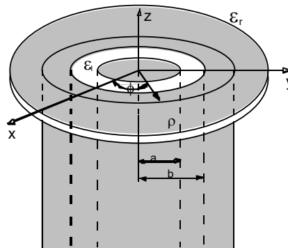
Figure 9.2.1.1. An open-ended coaxial probe with inner and outer radii a and b , respectively
