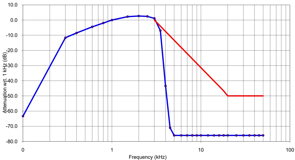
Audio Frequency Response 25 kHz Channel Spacing
