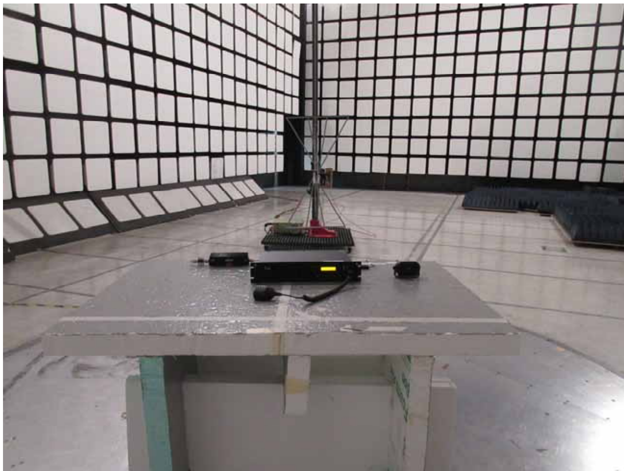
Radiated Setup
