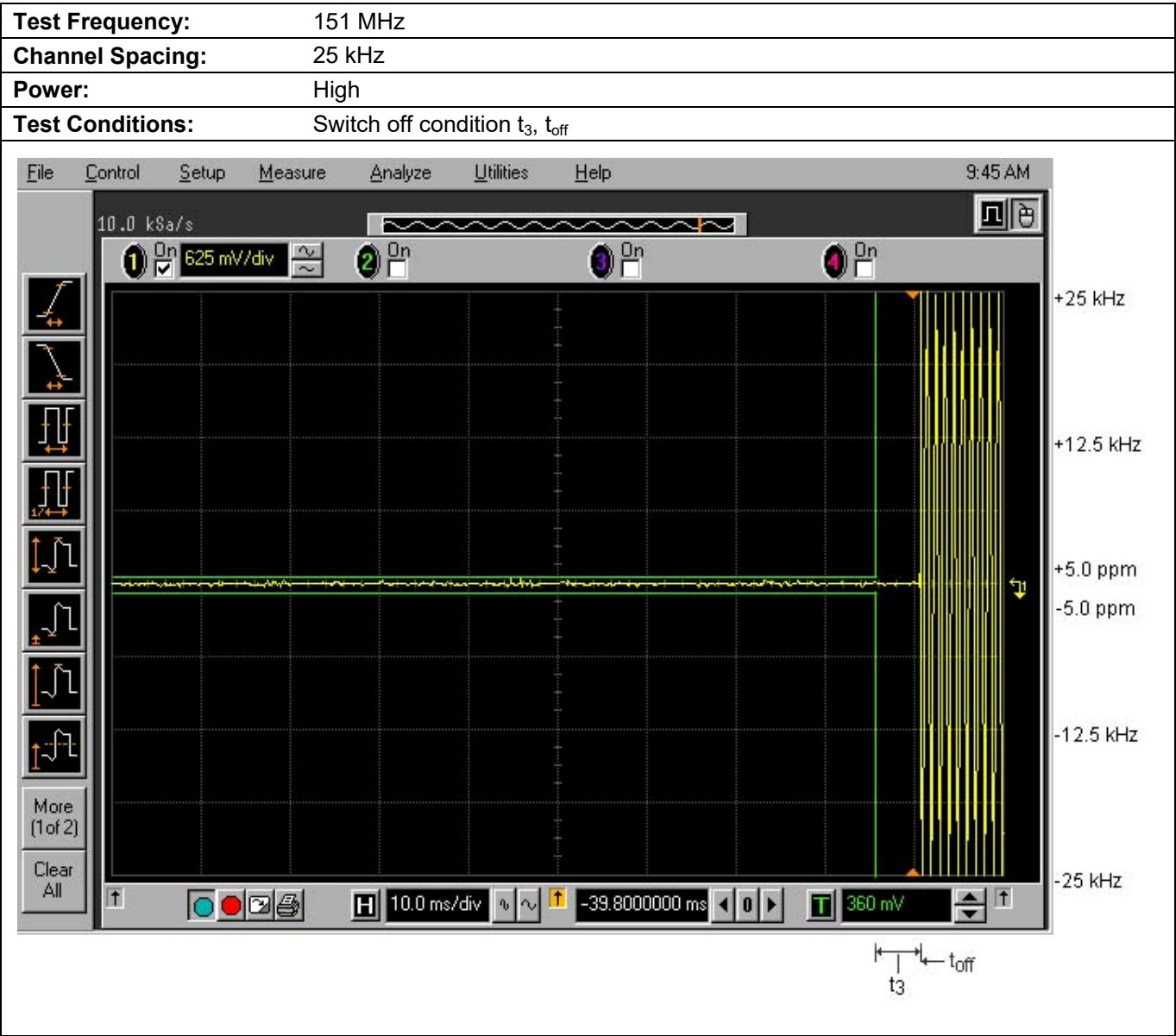
Plot 5.12.3.4. Transient Frequency Behavior for 25 kHz Channel Spacing
