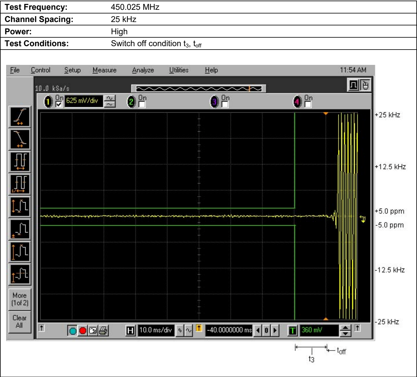
Plot 5.12.4.6. Transient Frequency Behavior for 25 kHz Channel Spacing
