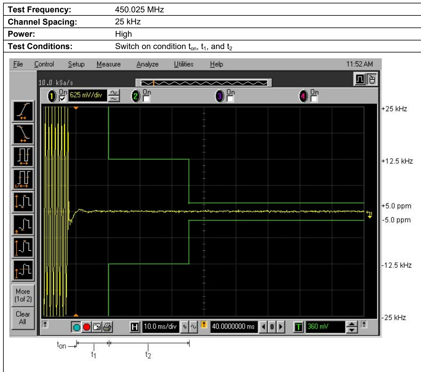
Plot 5.12.4.5. Transient Frequency Behavior for 25 kHz Channel Spacing
