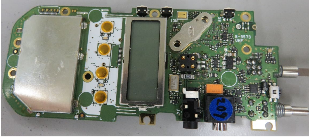
MAIN Board side-A view(IC-F2100DS)
