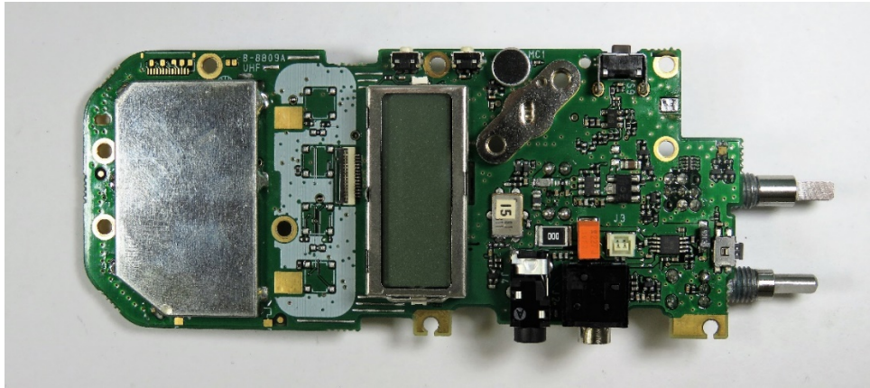
MAIN Board side-A view(IC-F2100DT)
