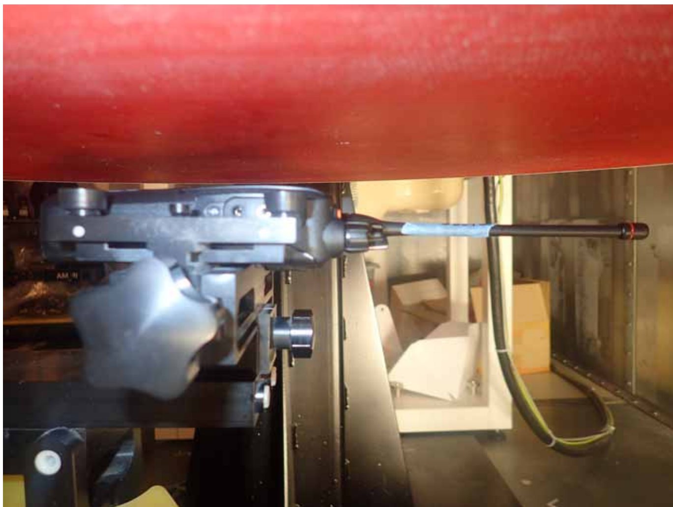
<Face Frontal Position, FA-SC57U Antenna, BP-280 battery pack>
