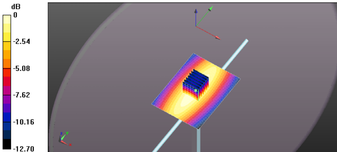
0 dB = 1.36 W/kg = 1.33 dBW/kg
