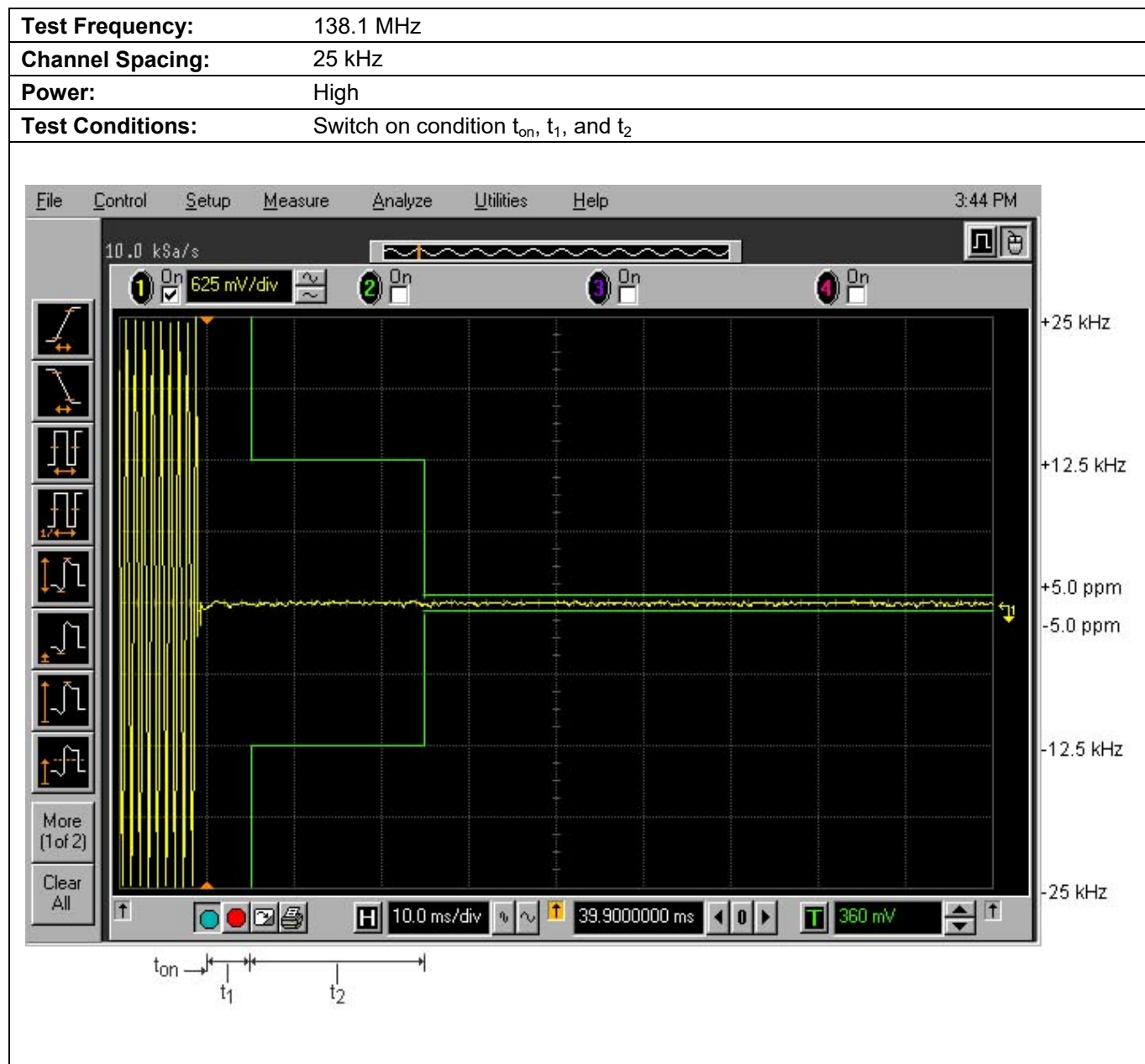
Plot 5.12.3.5. Transient Frequency Behavior for 25 kHz Channel Spacing
