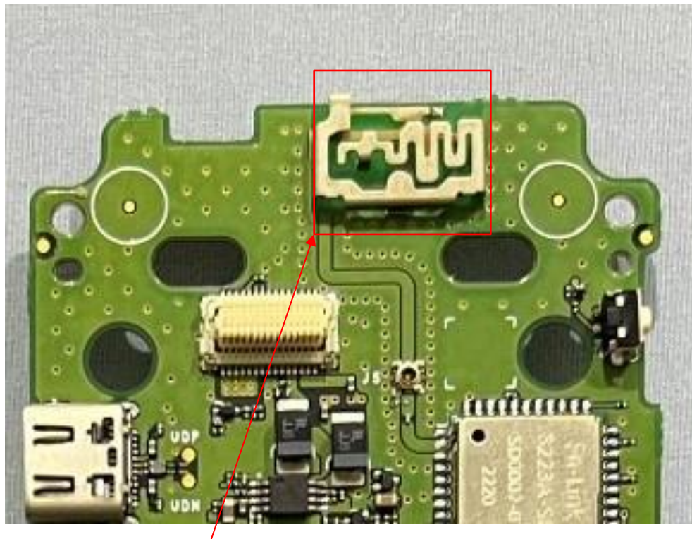
WiFi Antenna
