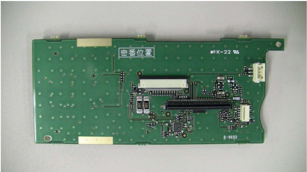
IC-F7540 FRONT-A UNIT B SIDE
