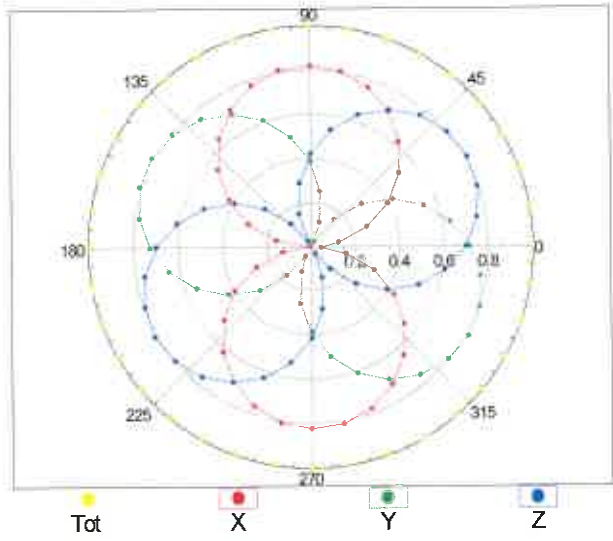
f=600 MHz,TEM
