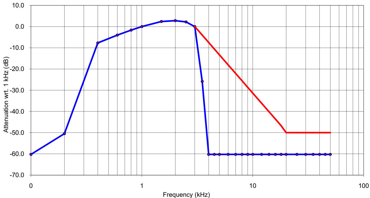
Audio Frequency Response 12.5 kHz Channel Spacing
