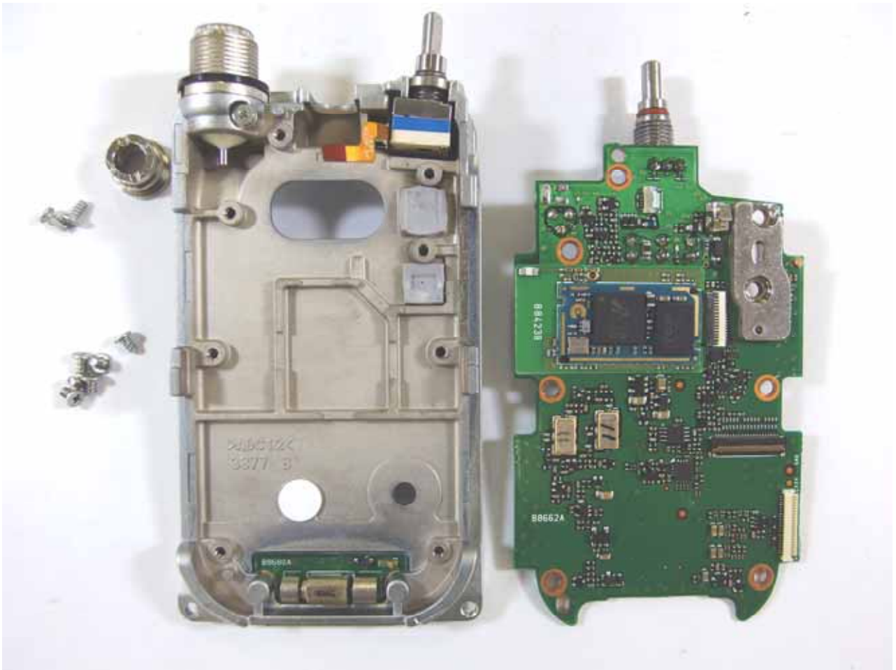
IC-F62D CHASSIS OPEN
