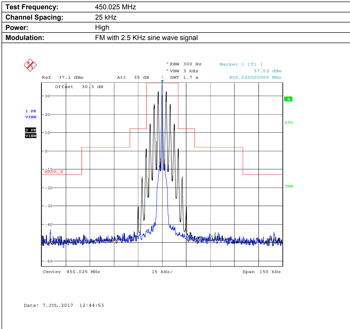
Plot 5.8.4.4.1. Emission Mask B, High Power
