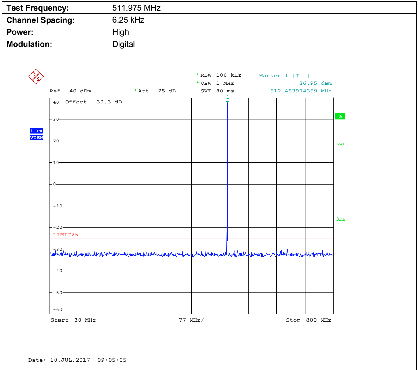
Plot 5.9.4.3.1. Conducted Transmitter Spurious Emissions for 511.975 MHz, High Power
