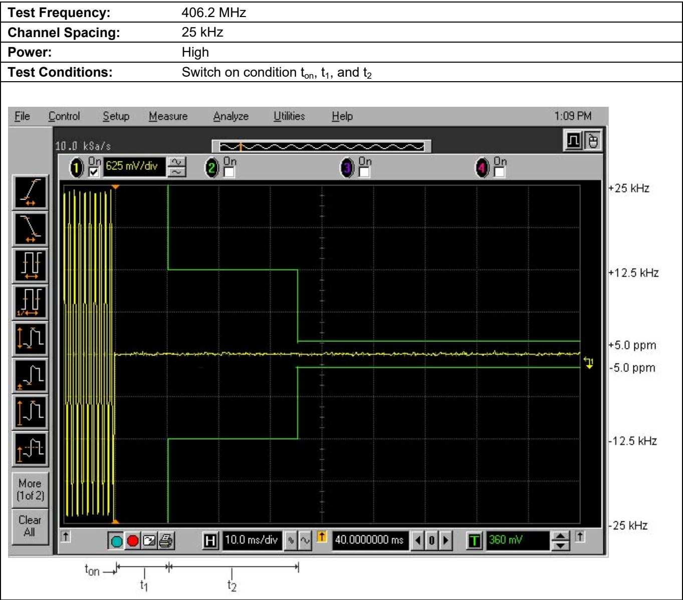
Plot 5.15.3.5. Transient Frequency Behavior for 25 kHz Channel Spacing
