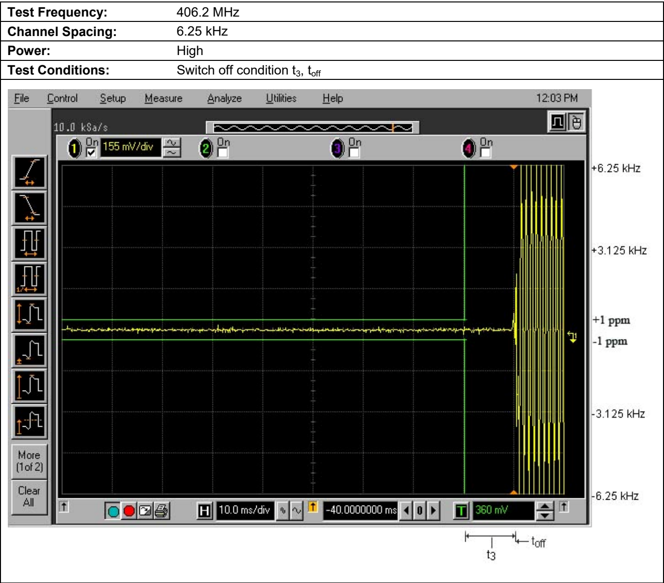
Plot 5.15.3.2. Transient Frequency Behavior for 6.25 kHz Channel Spacing
