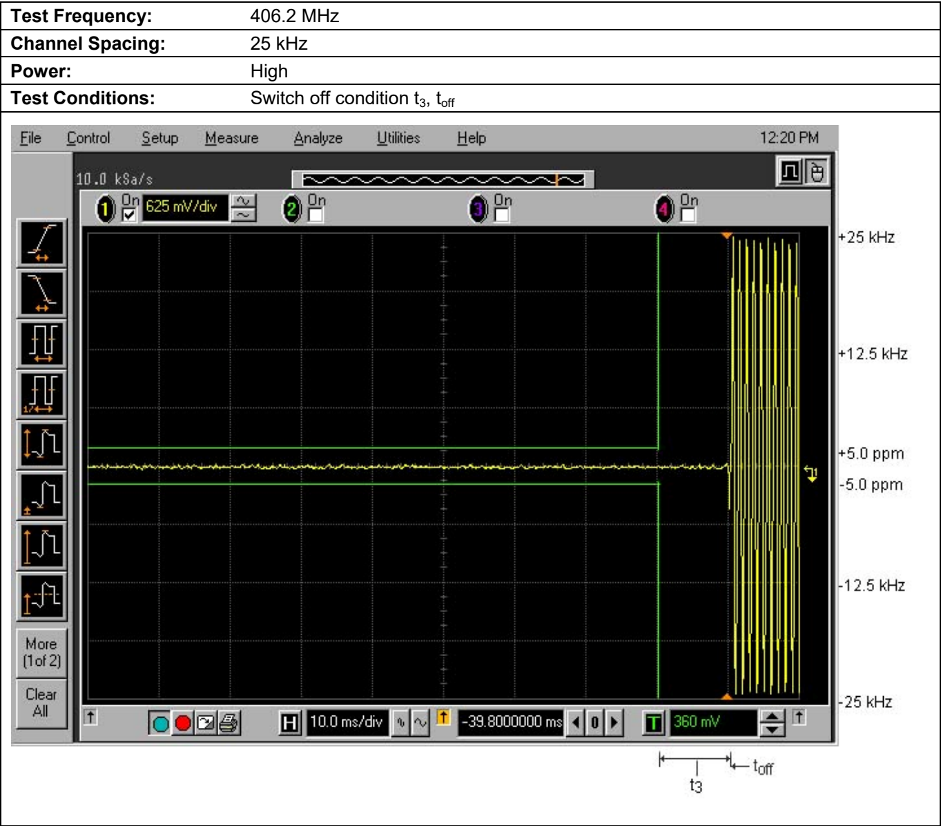
Plot 5.15.3.6. Transient Frequency Behavior for 25 kHz Channel Spacing
