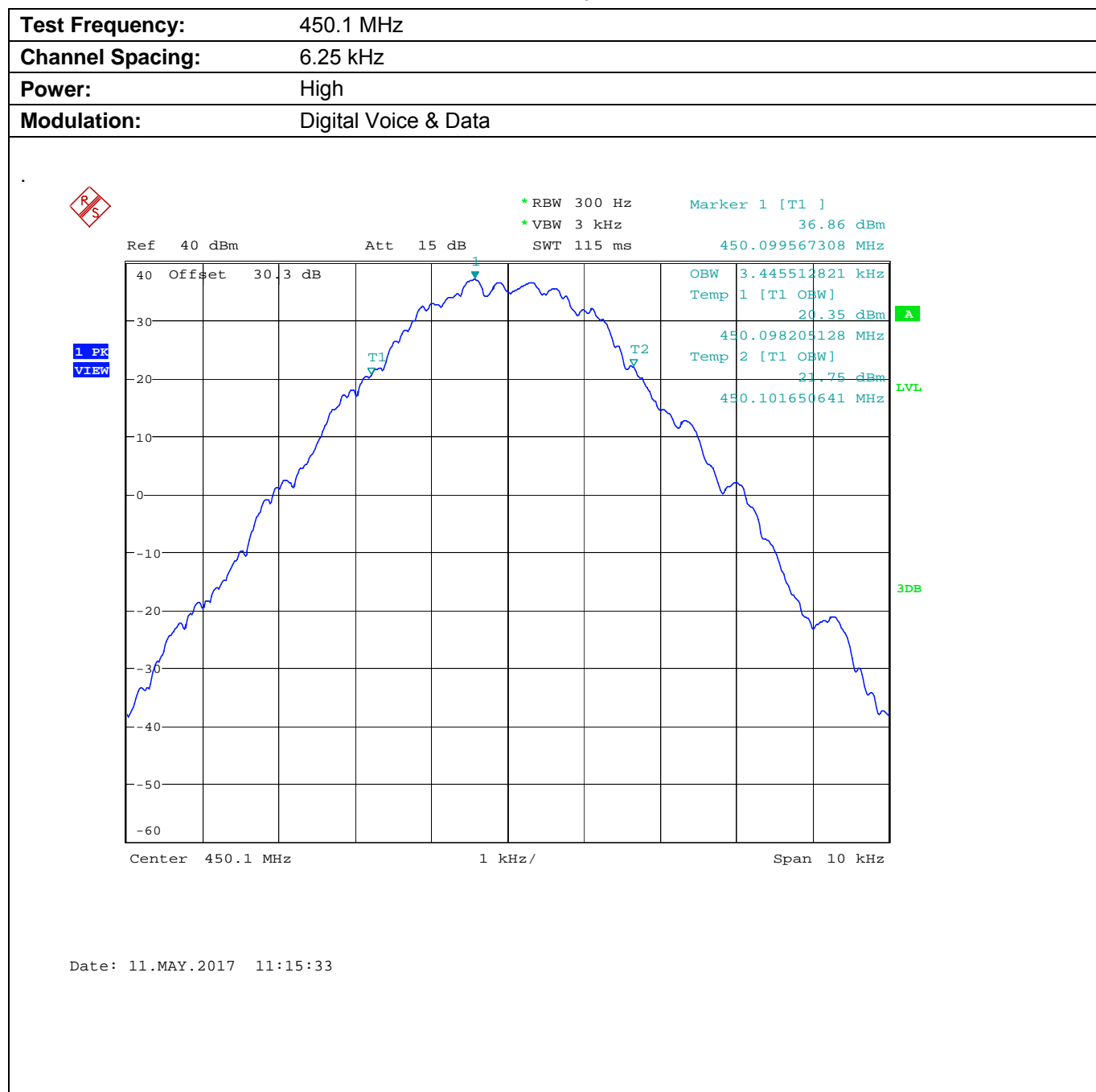
Plot 5.8.4.1.11. Occupied Bandwidth
