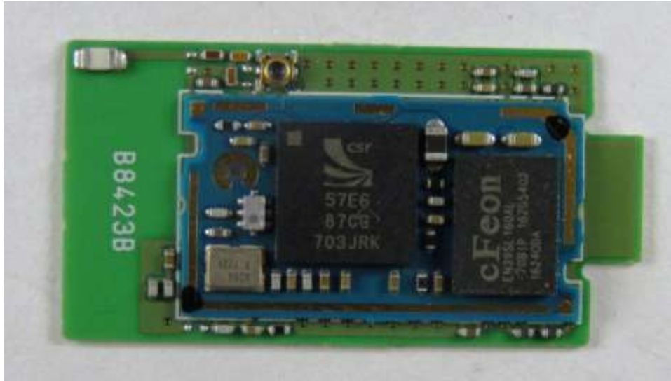
IC-F7510 Board(UT-136) on RELAY-A UNIT A SIDE
