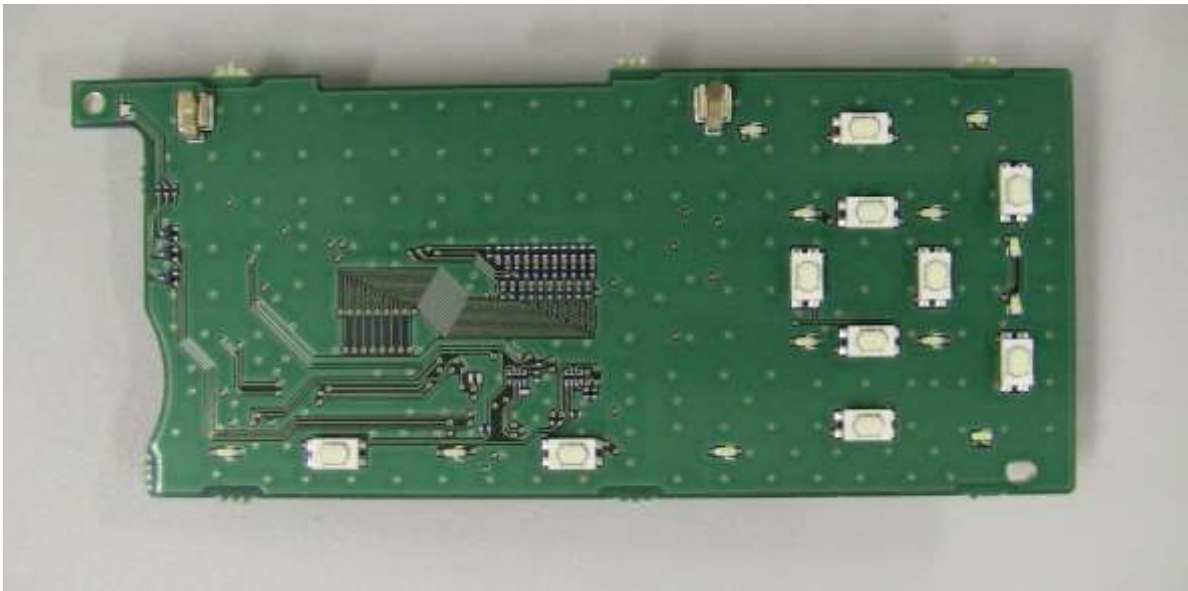
IC-F7510 FRONT-A UNIT A SIDE
