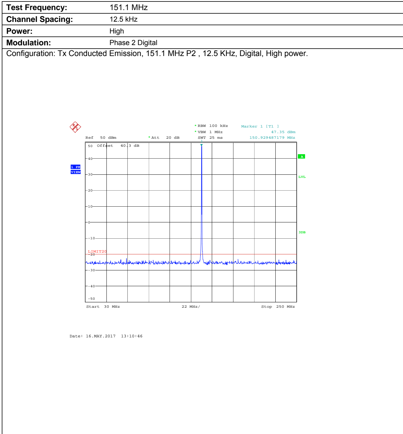
Plot 5.9.4.2.1. Conducted Transmitter Spurious Emissions for 151.1 MHz, High Power
