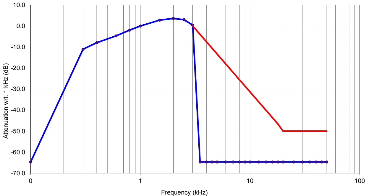
Audio Frequency Response 25 kHz Channel Spacing
