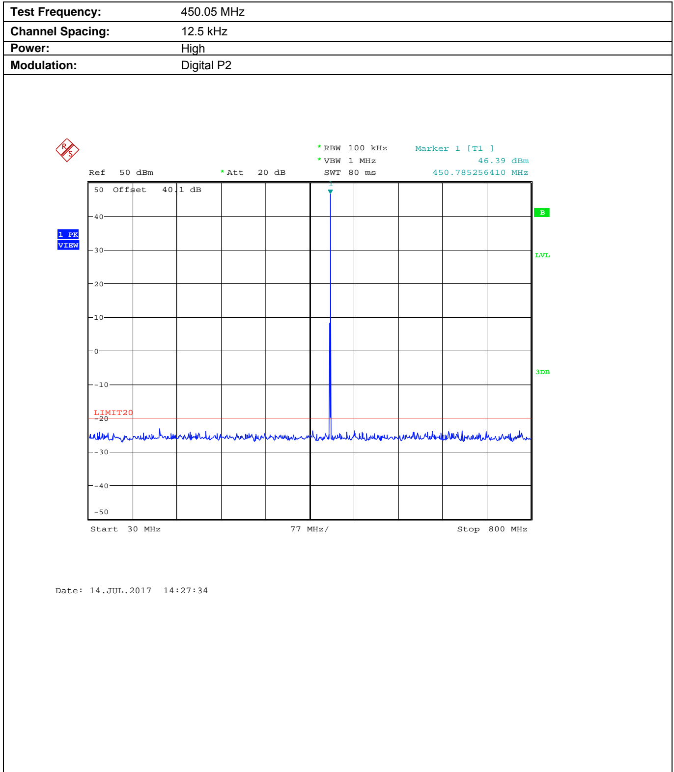
Plot 5.9.4.1.1. Conducted Transmitter Spurious Emissions for 450.05 MHz, High Power,
