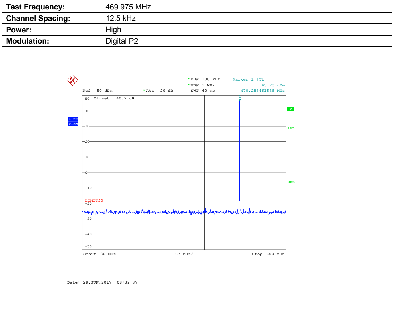
Plot 5.9.4.3.1. Conducted Transmitter Spurious Emissions for 469.975 MHz, High Power
