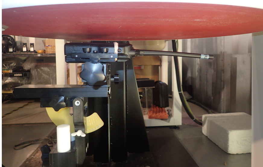
< FA-S82V Antenna >
