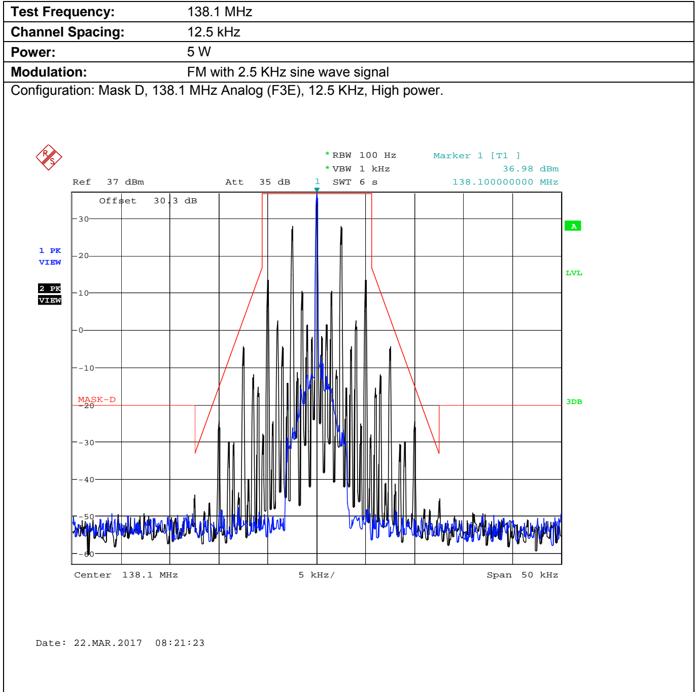
Plot 5.8.4.2.1. Emission Mask D, High Power
