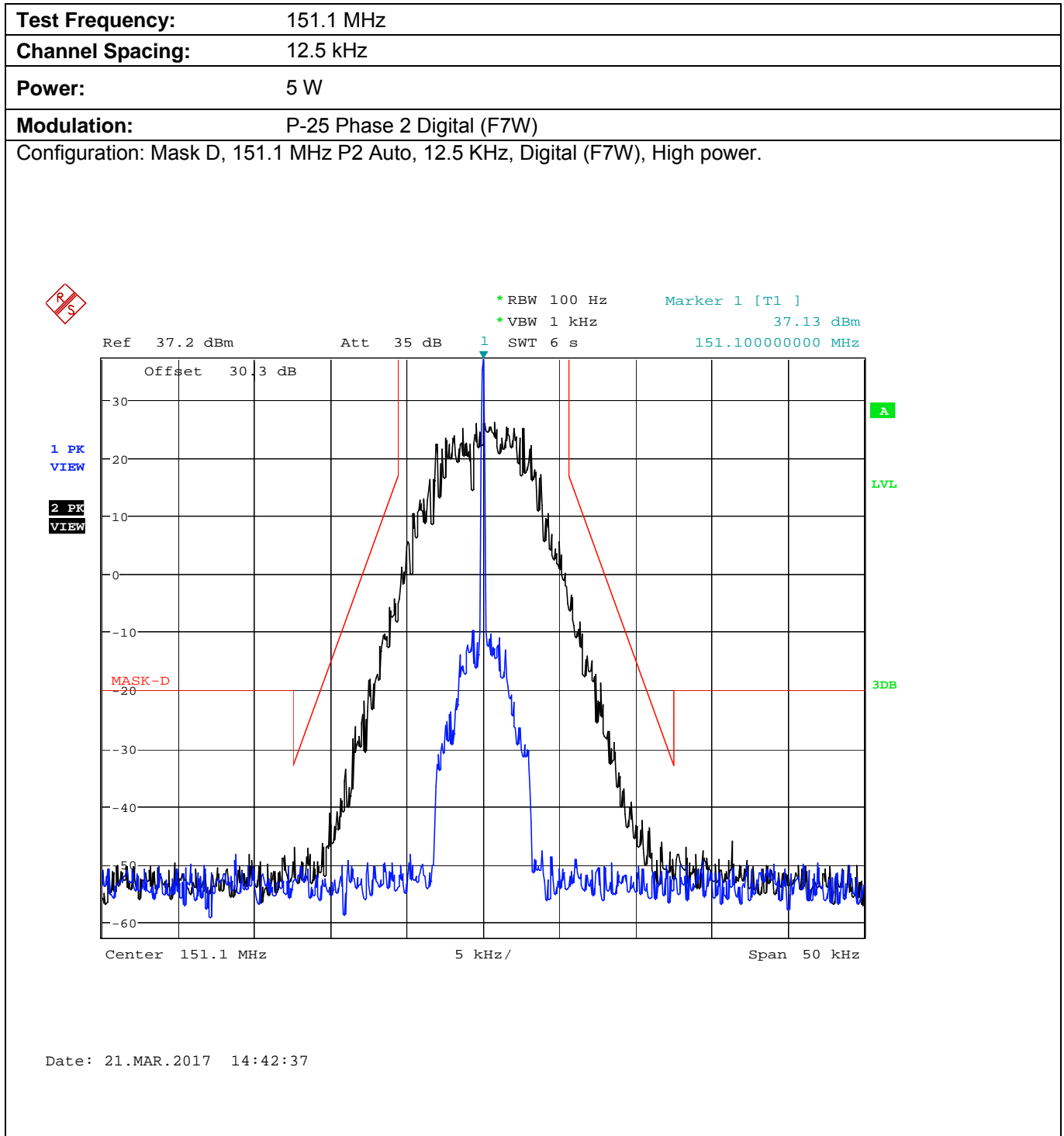
Plot 5.8.4.2.14. Emission Mask D, High Power
