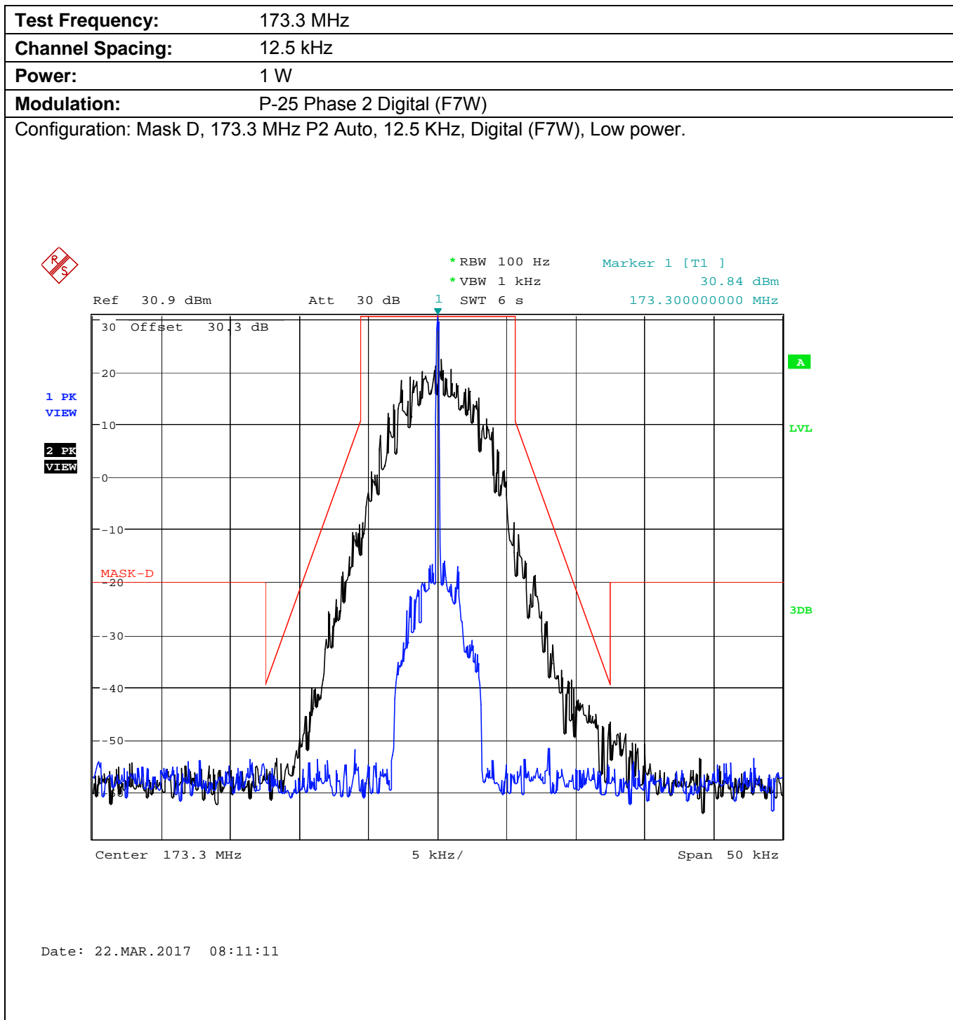
Plot 5.8.4.2.18. Emission Mask D, Low Power
