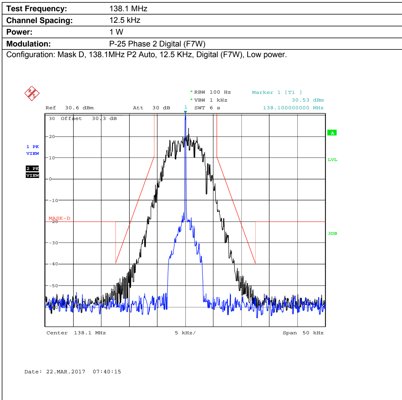
Plot 5.8.4.2.16. Emission Mask D, Low Power
