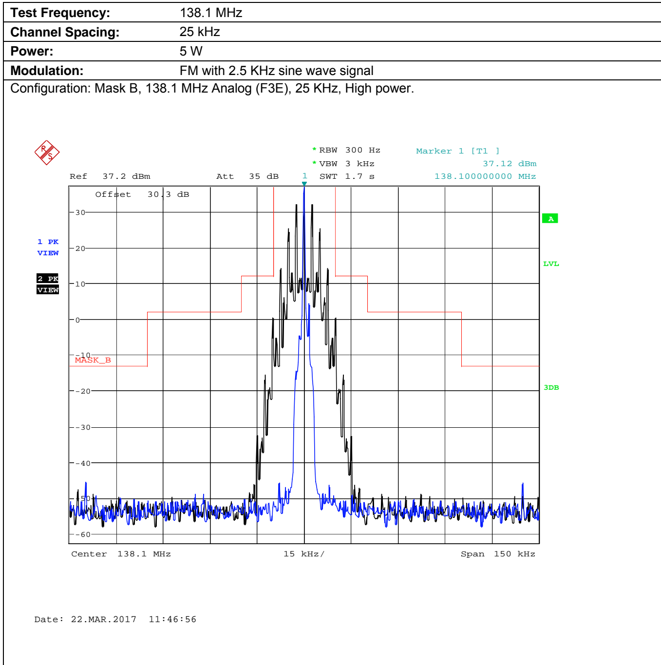
Plot 5.8.4.3.1. Emission Mask B, High Power
