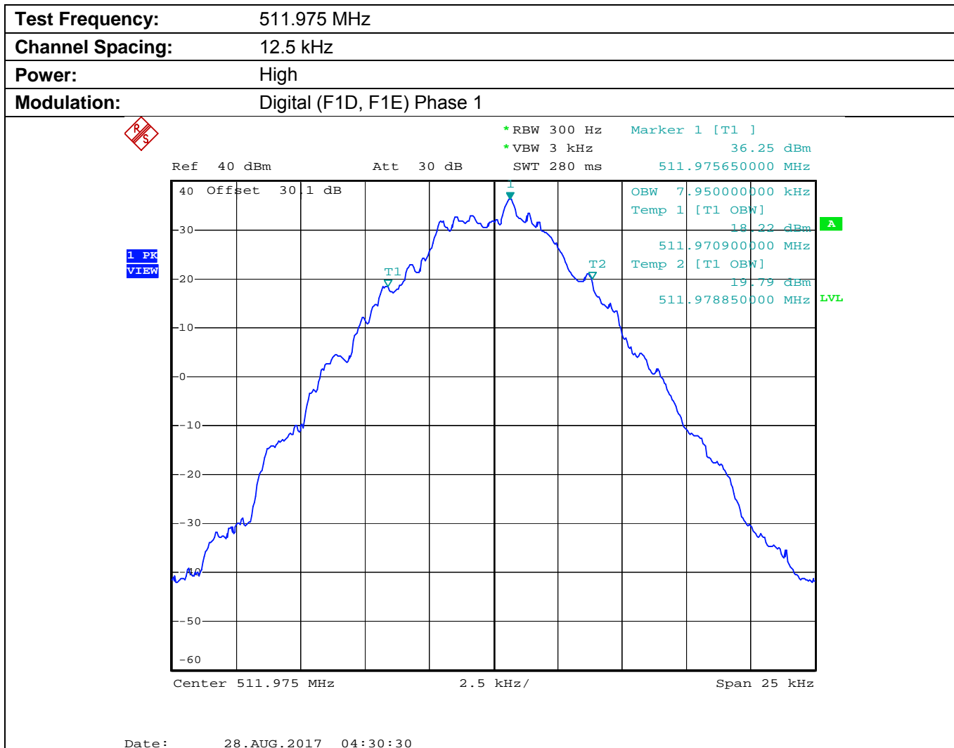
Plot 5.8.4.1.9. Occupied Bandwidth
