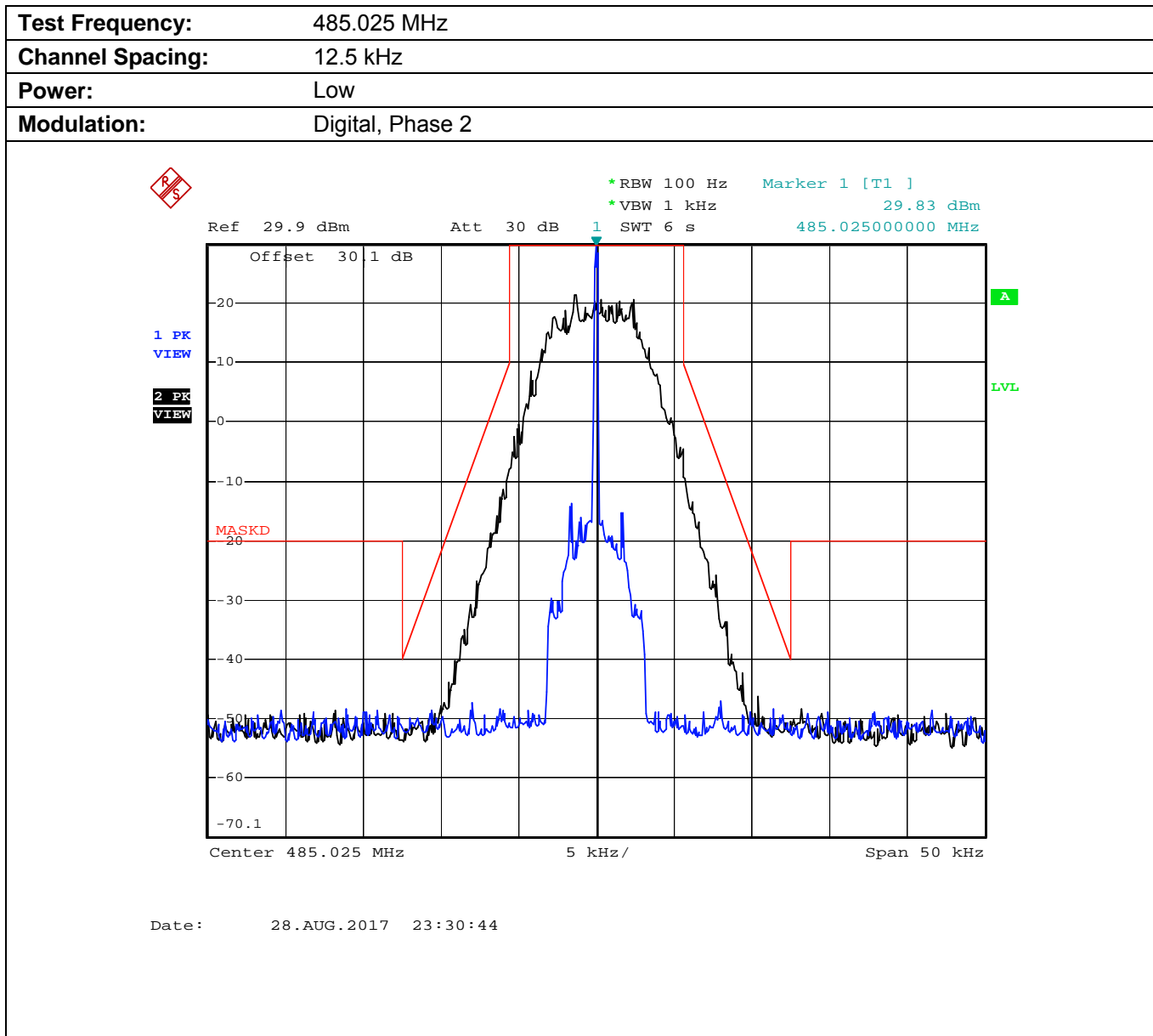
Plot 5.8.4.2.17. Emission Mask D, Low Power
