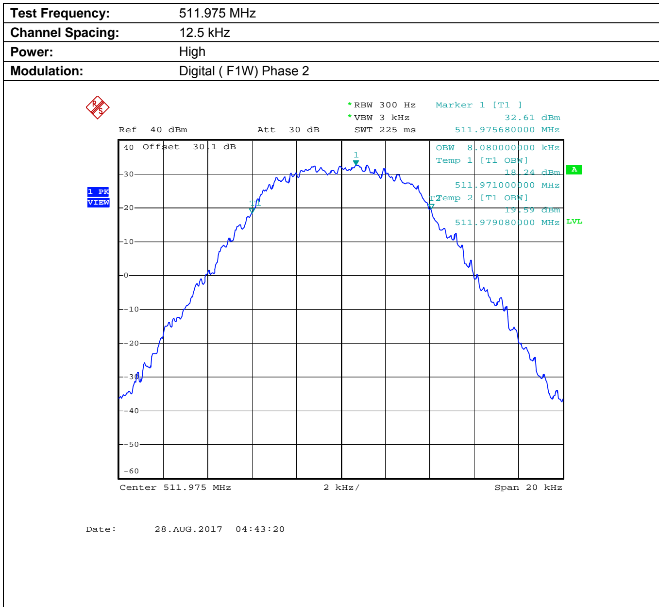
Plot 5.8.4.1.12. Occupied Bandwidth
