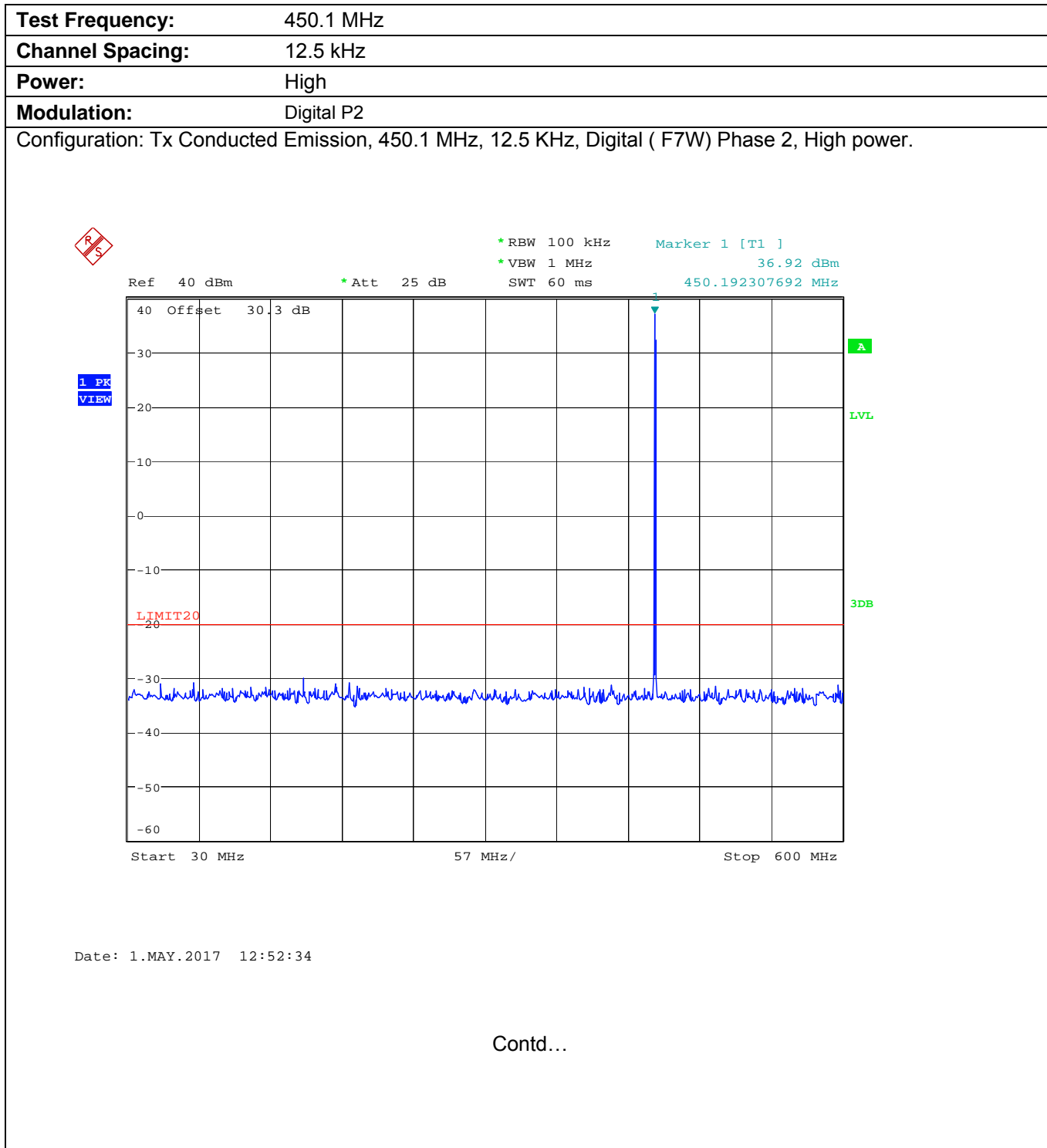
Plot 5.9.4.2.1. Conducted Transmitter Spurious Emissions for 450.1 MHz, High Power
