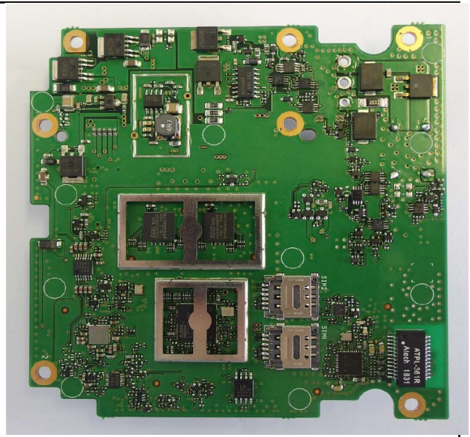
Main Board – Rear View
