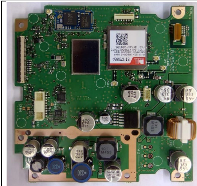
Main Board – Top View
