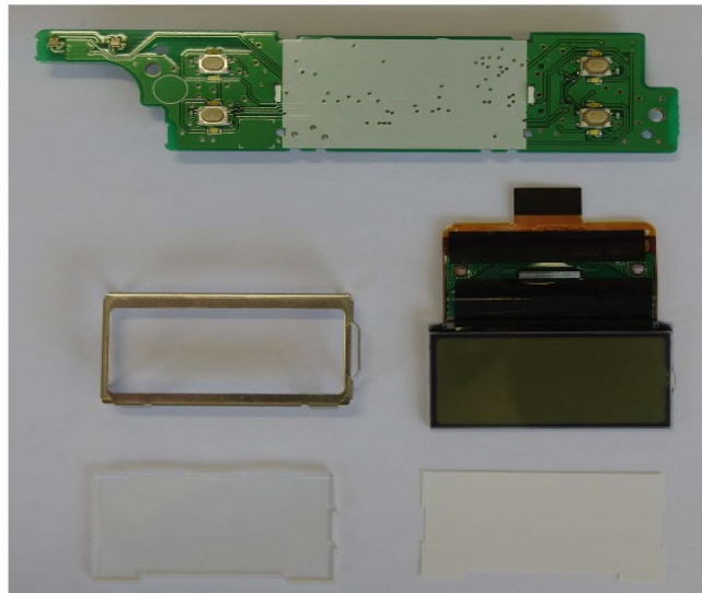
PCB 2 – Front View
